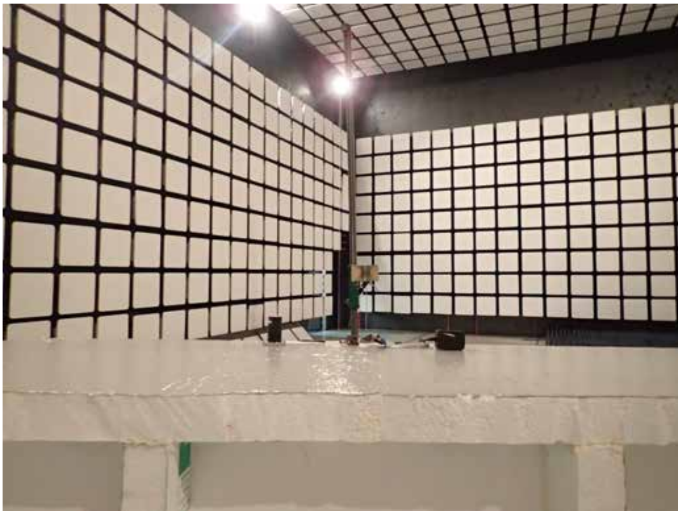
Radiated Emissions @ 3 m EUT with 4 dBi Puck Antenna, Orthogonal Position 2
