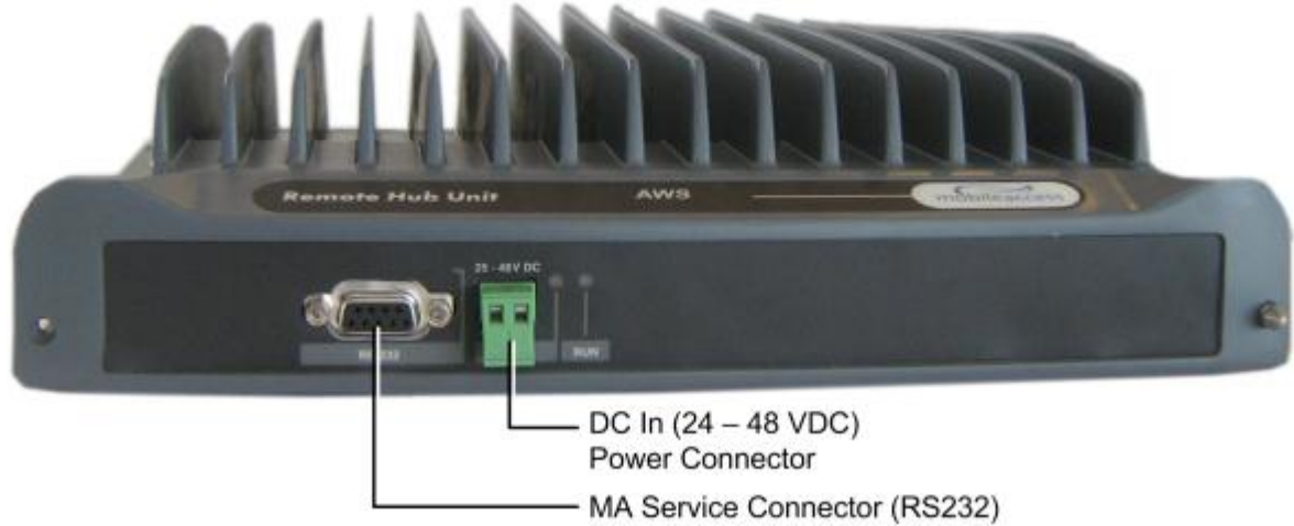
Figure 1. AWS1200 AO Front Panel
