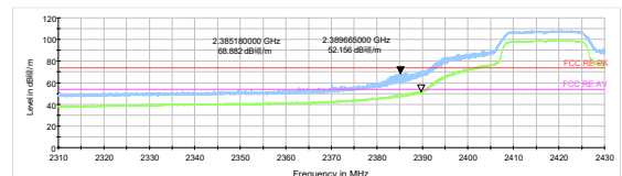
802.11n HT40 -Channel 2 Peak+ Average
