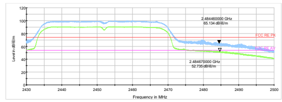
802.11n HT40 -Channel 9 Peak+ Average
