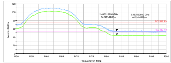
802.11b-Channel 11 Peak+ Average
