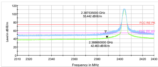
Bluetooth LE (2M) Channel 0 Peak+ Average
