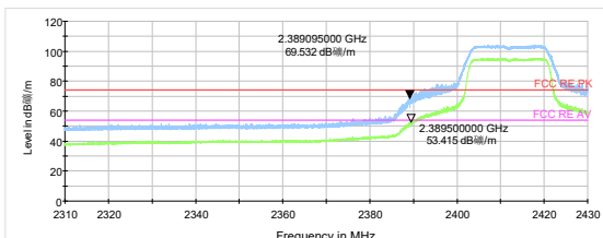
802.11n HT20 -Channel 1 Peak+ Average
