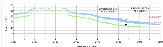
802.11g-Channel 8 Peak+ Average
