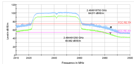
802.11n HT20 -Channel 7 Peak+ Average
