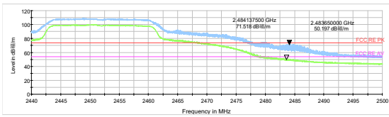
802.11n HT20 -Channel 9 Peak+ Average
