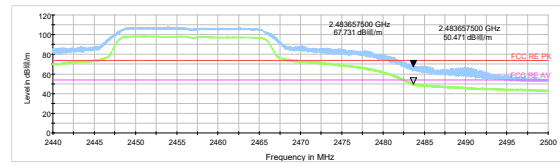
802.11n HT20 -Channel 10 Peak+ Average
