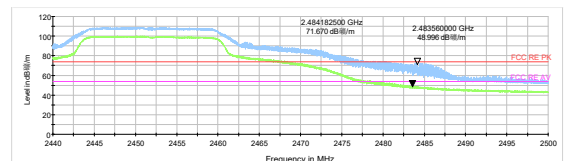
802.11g-Channel 9 Peak+ Average
