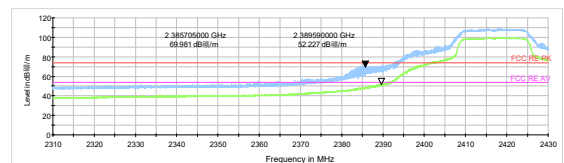
802.11g-Channel 2 Peak+ Average
