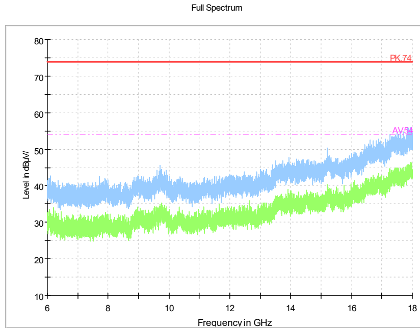
Pic11. Radiated emission (6GHz –18GHz)
