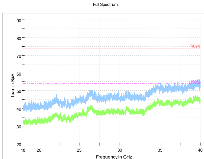
Pic12. Radiated emission (18GHz –40GHz)
