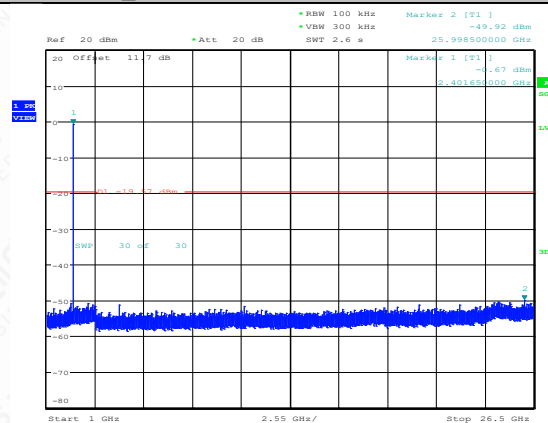
BLE_2M-Ant1-2402-1000~26500-PASS
