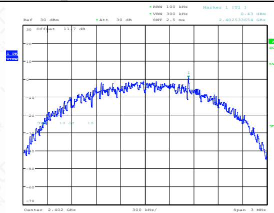
BLE_2M-Ant1-2402-0~Reference-PASS
