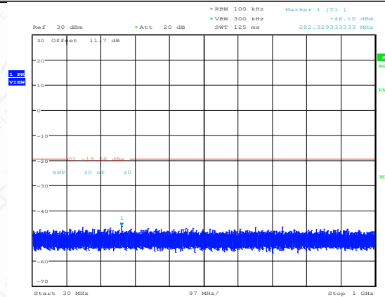
BLE_1M-Ant1-2480-30~1000-PASS
