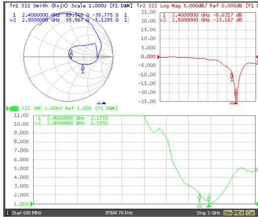
WIFI Antenna
