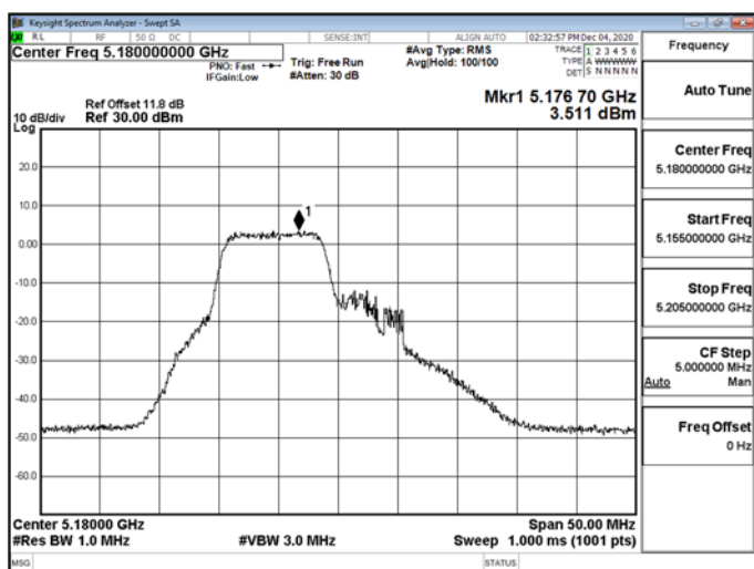
802.11ax_20MHz_RU_106_53_CH1_5180MHz-5180
