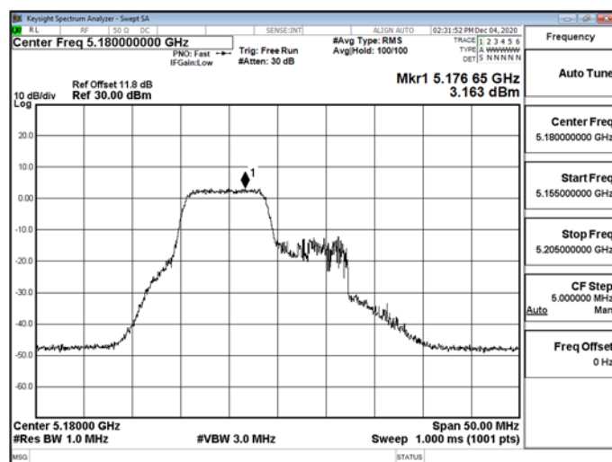
802.11ax_20MHz_RU_106_53_CH0_5180MHz-5180
