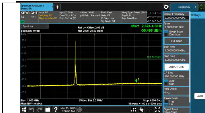
Band66-15MHz-QPSK-132047-1RB#74-1000~3000-PASS
