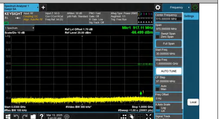
Band66-5MHz-QPSK-132647-1RB#24-30~1000-PASS
