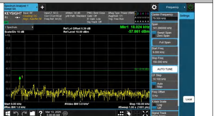
Band66-5MHz-QPSK-132647-1RB#24-0.009~0.15-PASS
