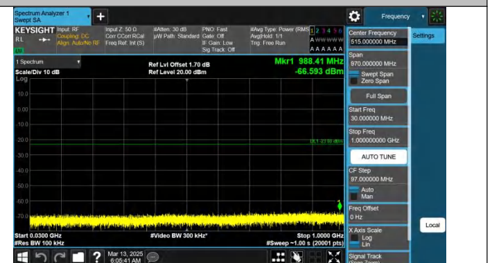
Band66-20MHz-QPSK-132072-1RB#99-30~1000-PASS
