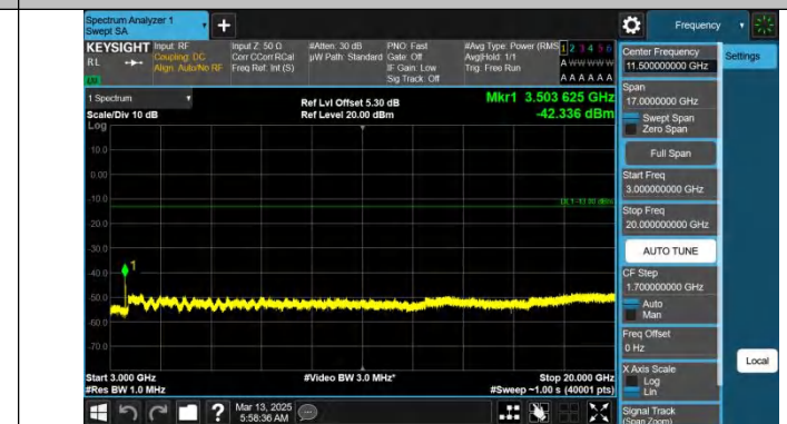
Band66-15MHz-QPSK-132322-1RB#74-3000~20000-PASS
