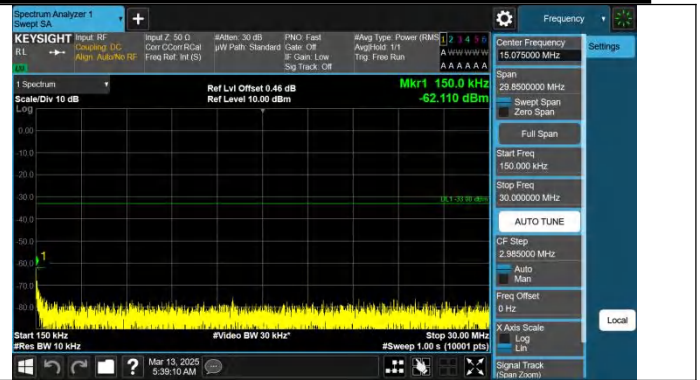
Band66-5MHz-QPSK-132647-1RB#0-0.15~30-PASS
