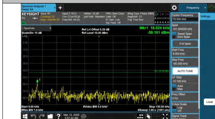
Band66-15MHz-QPSK-132322-1RB#0-0.009~0.15-PASS
