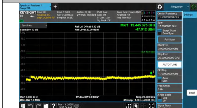
Band66-15MHz-QPSK-132322-1RB#0-3000~20000-PASS
