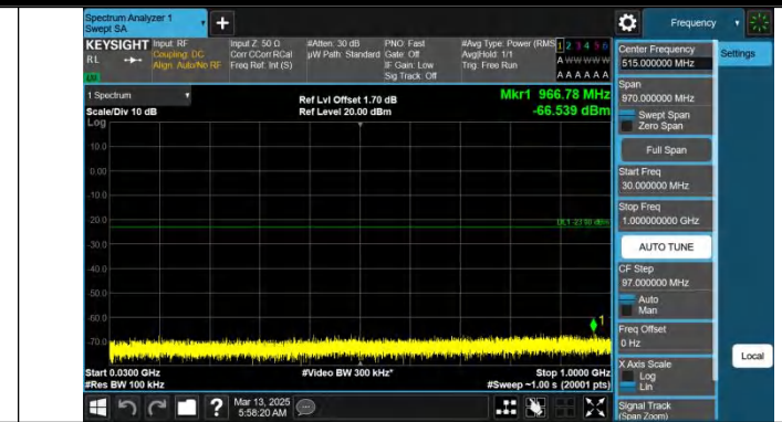
Band66-15MHz-QPSK-132322-1RB#74-30~1000-PASS
