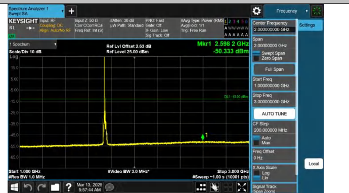
Band66-15MHz-QPSK-132322-1RB#0-1000~3000-PASS
