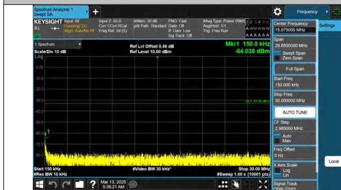
Band66-5MHz-QPSK-132322-1RB#24-0.15~30-PASS
