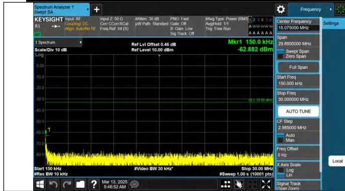
Band66-10MHz-QPSK-132022-1RB#49-0.15~30-PASS
