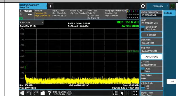
Band66-15MHz-QPSK-132597-1RB#0-0.15~30-PASS
