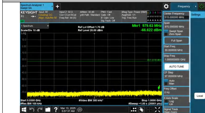
Band66-15MHz-QPSK-132322-1RB#0-30~1000-PASS
