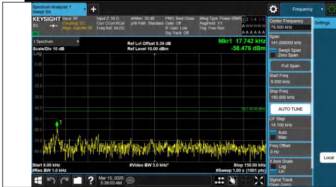
Band66-5MHz-QPSK-132647-1RB#0-0.009~0.15-PASS
