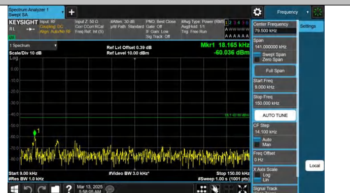
Band66-15MHz-QPSK-132322-1RB#74-0.009~0.15-PASS
