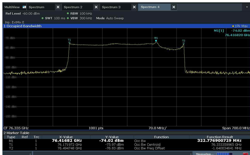
Occupied Bandwidth
