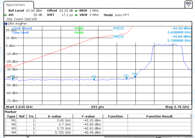
11AC20SISO-Ant1-5745-PASS
