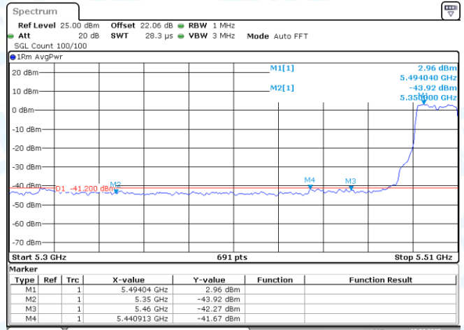
11AX20SISO-Ant1-5500-PASS
