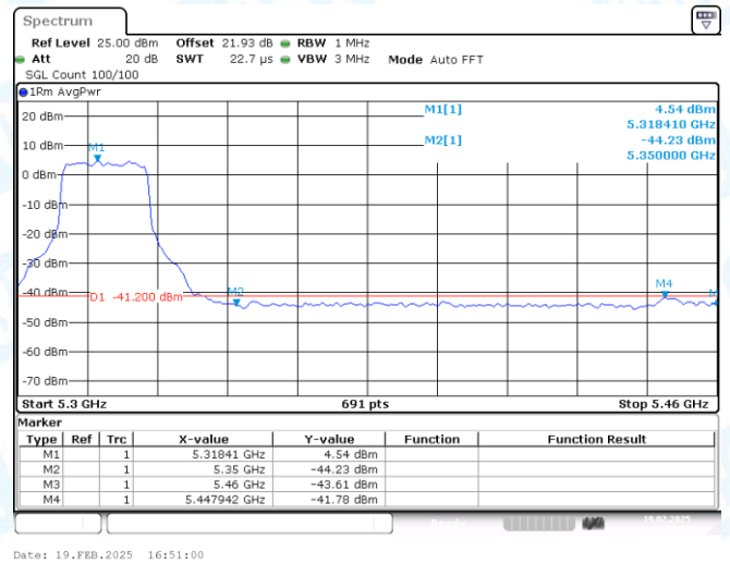
11AX20SISO-Ant1-5320-PASS
