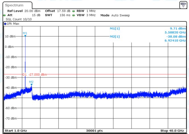
11AX20SISO-Ant1-5500-1000~40000-PASS
