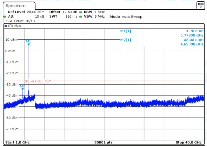
11AX20SISO-Ant1-5745-1000~40000-PASS
