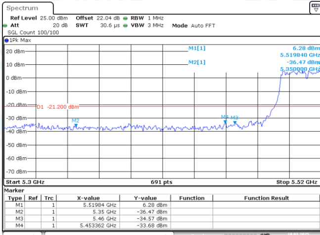
11N40SISO-Ant1-5510-PASS
