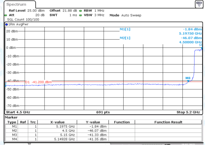
11AX40SISO-Ant1-5190-PASS
