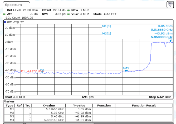
11AC40SISO-Ant1-5310-PASS
