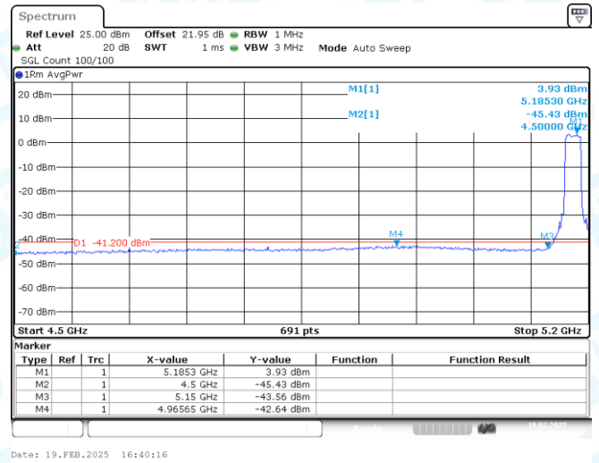
11AX20SISO-Ant1-5180-PASS
