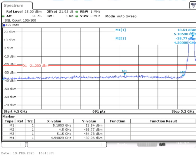
11AX20SISO-Ant1-5180-PASS
