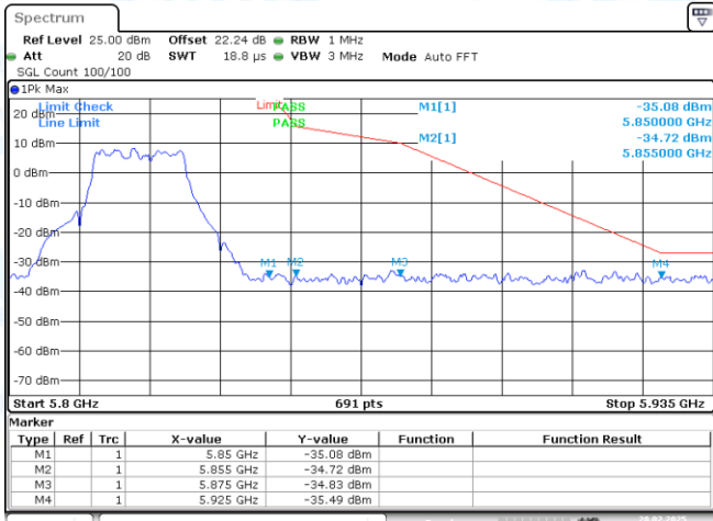
11N20SISO-Ant1-5825-PASS
