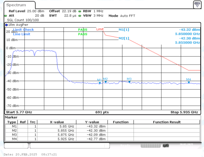
11AC40SISO-Ant1-5795-PASS
