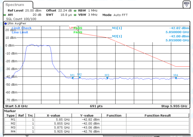
11N20SISO-Ant1-5825-PASS
