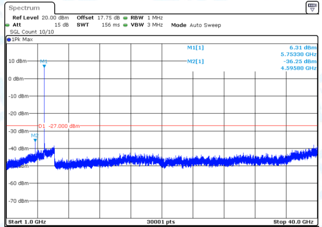
11AX20SISO-Ant1-5745-1000~40000-PASS
