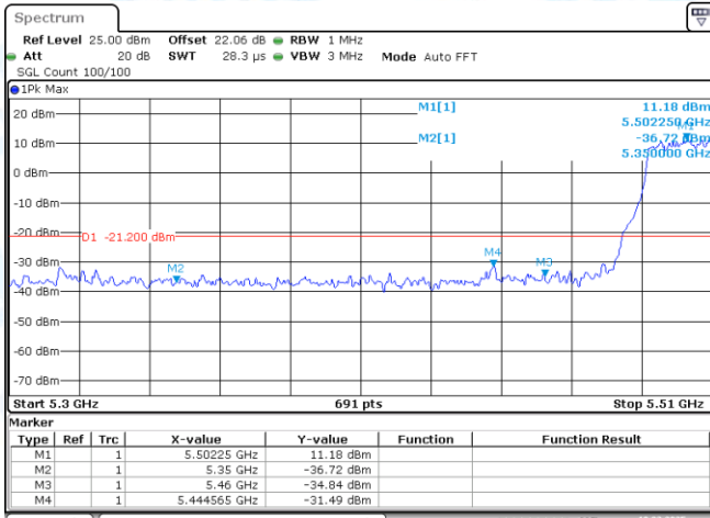
11AX20SISO-Ant1-5500-PASS
