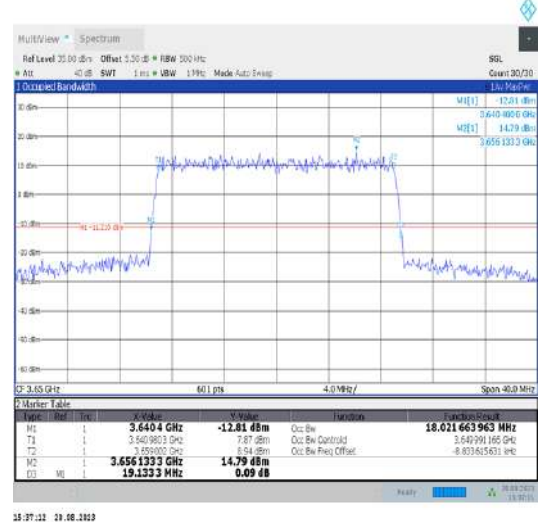
Band43-20MHz-16QAM-44090-100RB#0-PASS
