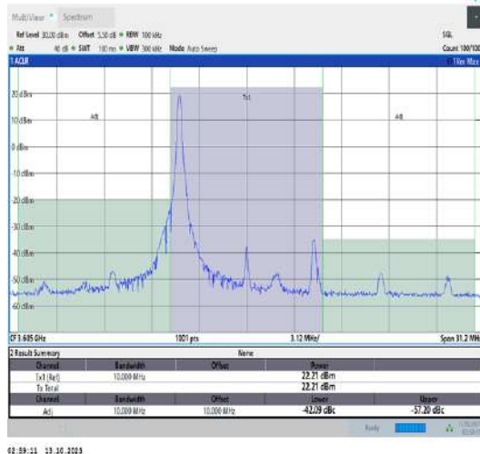
43(3600-3700)-10MHz-QPSK-43640-1RB#0-PASS
