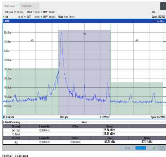
43(3600-3700)-10MHz-QPSK-44090-1RB#0-PASS
