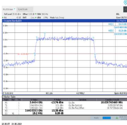
Band43-20MHz-QPSK-44090-100RB#0-PASS
