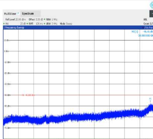
Band43_20MHz_QPSK_44090_1RB#0_1000~3000_1000~3000
