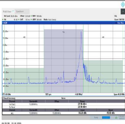
43(3600-3700)-15MHz-QPSK-44090-1RB#74-PASS
