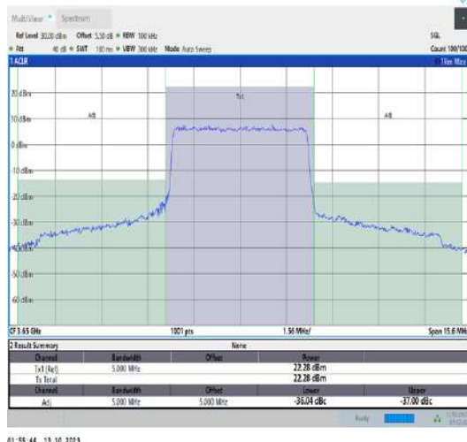
43(3600-3700)-5MHz-QPSK-44090-25RB#0-PASS
