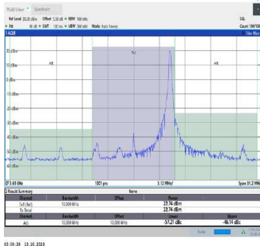
43(3600-3700)-10MHz-QPSK-44090-1RB#49-PASS
