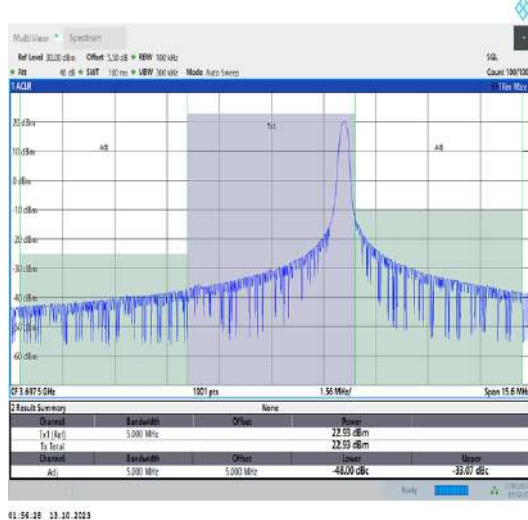
43(3600-3700)-5MHz-QPSK-44565-1RB#24-PASS
