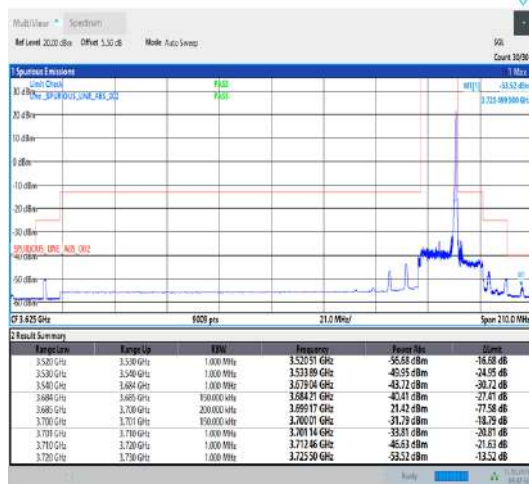
Band43_15MHz_QPSK_44515_1RB#74
