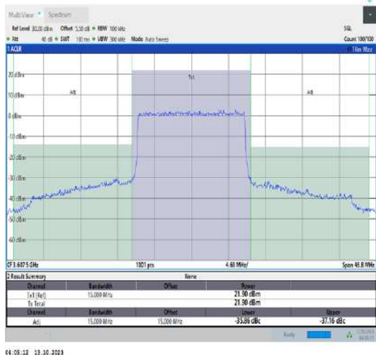
43(3600-3700)-15MHz-QPSK-43665-75RB#0-PASS
