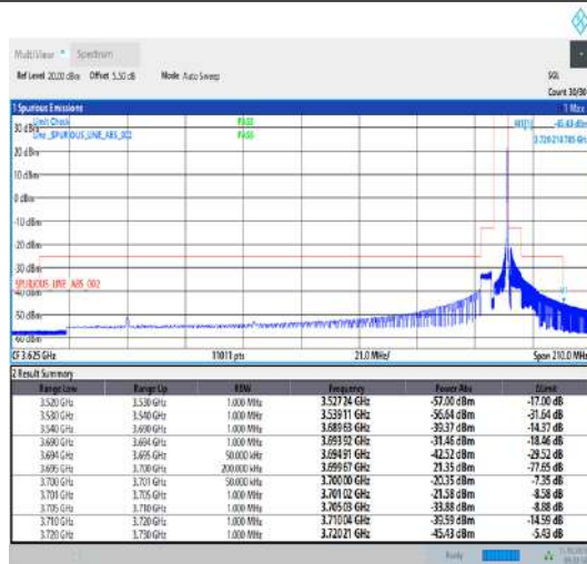
Band43_5MHz_QPSK_43615_1RB#0
