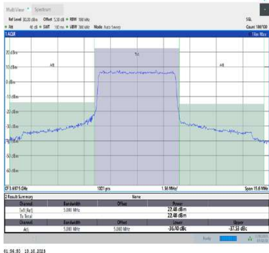
43(3600-3700)-5MHz-QPSK-44565-25RB#0-PASS
