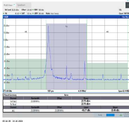
43(3600-3700)-20MHz-QPSK-44490-1RB#0-PASS
