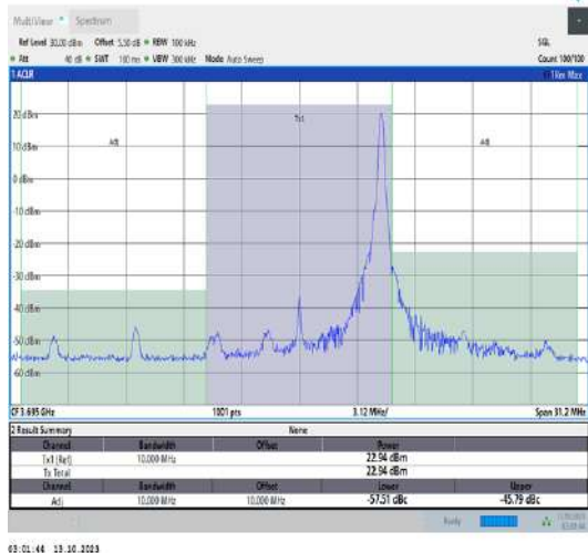
43(3600-3700)-10MHz-QPSK-44540-1RB#49-PASS
