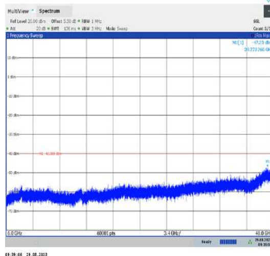
Band43_20MHz_QPSK_43690_1RB#0_6000~40000_6000~40000
