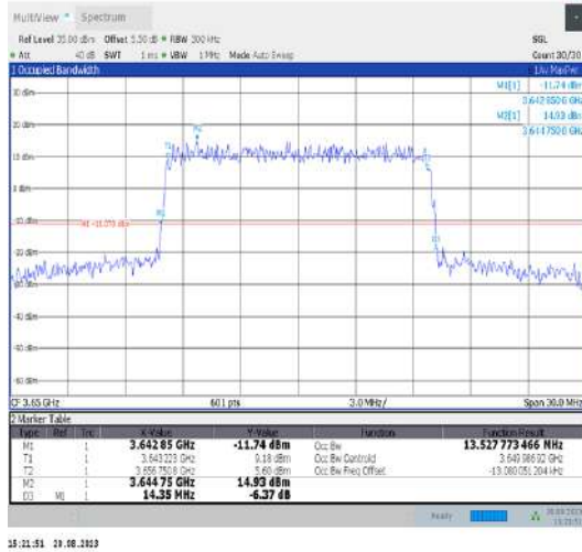
Band43-15MHz-QPSK-44090-75RB#0-PASS
