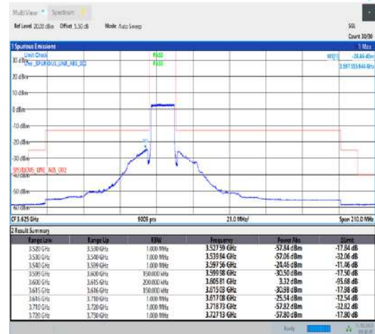
Band43_15MHz_QPSK_43665_75RB#0
