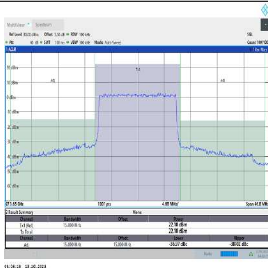
43(3600-3700)-15MHz-QPSK-44090-75RB#0-PASS
