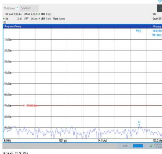
Band43_20MHz_QPSK_44090_1RB#0_0.009~0.15_0.009~0.15
