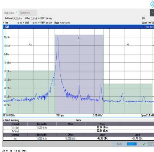
43(3600-3700)-10MHz-QPSK-44540-1RB#0-PASS
