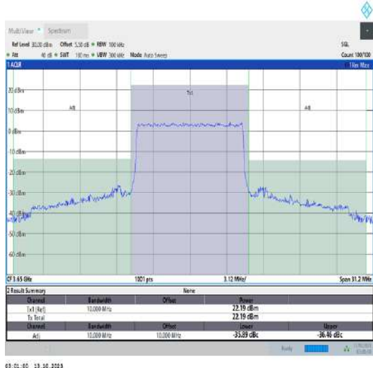
43(3600-3700)-10MHz-QPSK-44090-50RB#0-PASS
