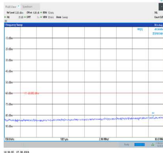
Band43_20MHz_QPSK_44490_1RB#0_0.15~30_0.15~30
