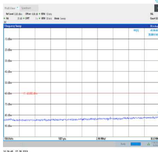
Band43_20MHz_QPSK_44090_1RB#0_0.15~30_0.15~30
