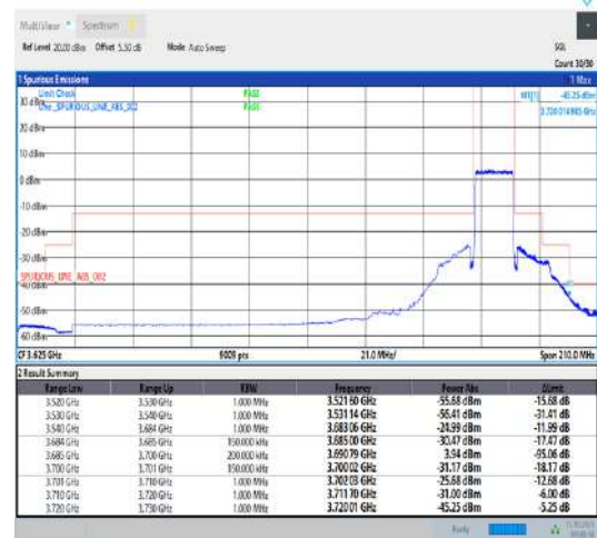
Band43_15MHz_QPSK_44515_75RB#0
