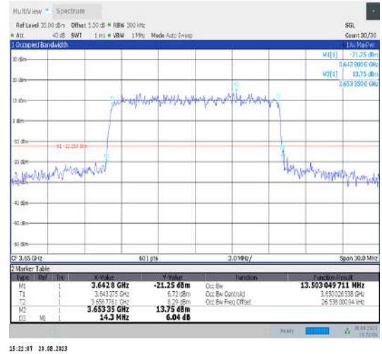
Band43-15MHz-16QAM-44090-75RB#0-PASS
