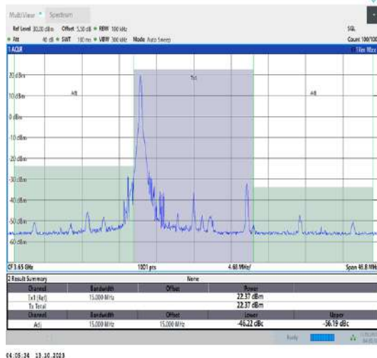
43(3600-3700)-15MHz-QPSK-44090-1RB#0-PASS
