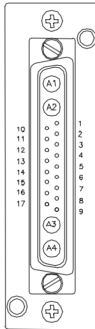
Figure 2-2. DC and Logic Connector (on Rear of G3S-1900-80 Amplifier Module)
