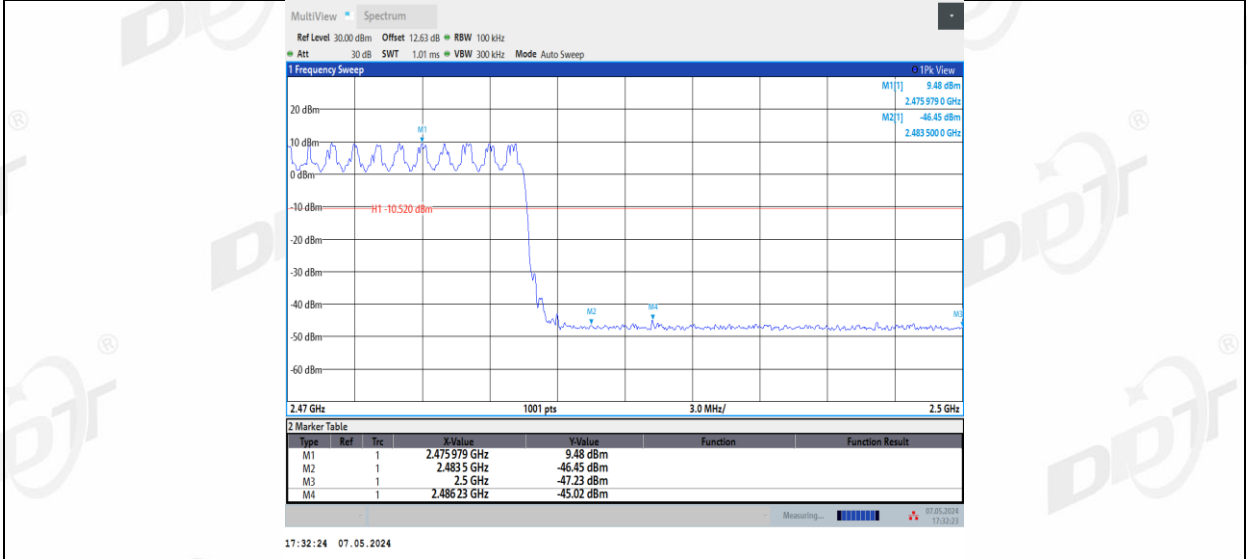
2DH5_Ant2_R_High_Hop_2480
