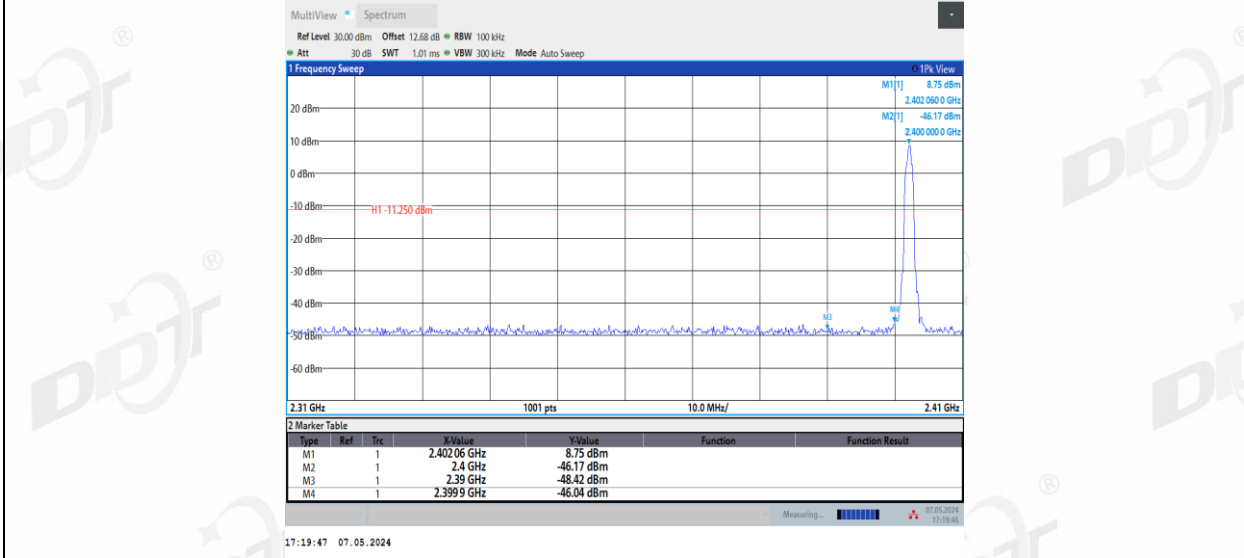
3DH5_Ant2_R_Low_2402
