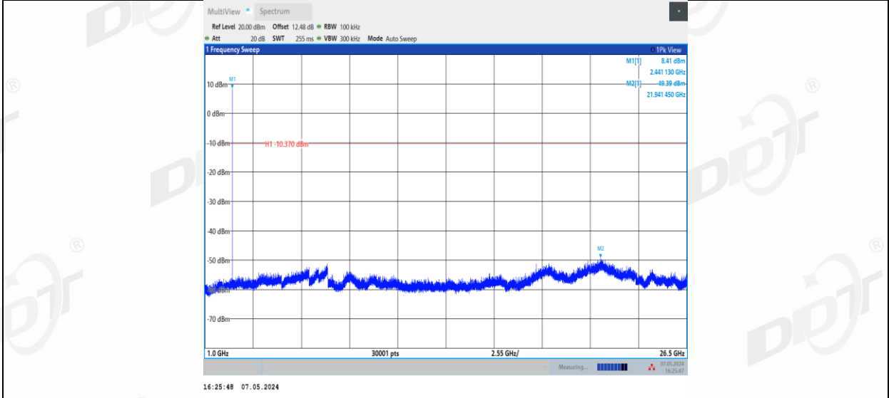
2DH5_Ant1_L_2480_0~Reference
