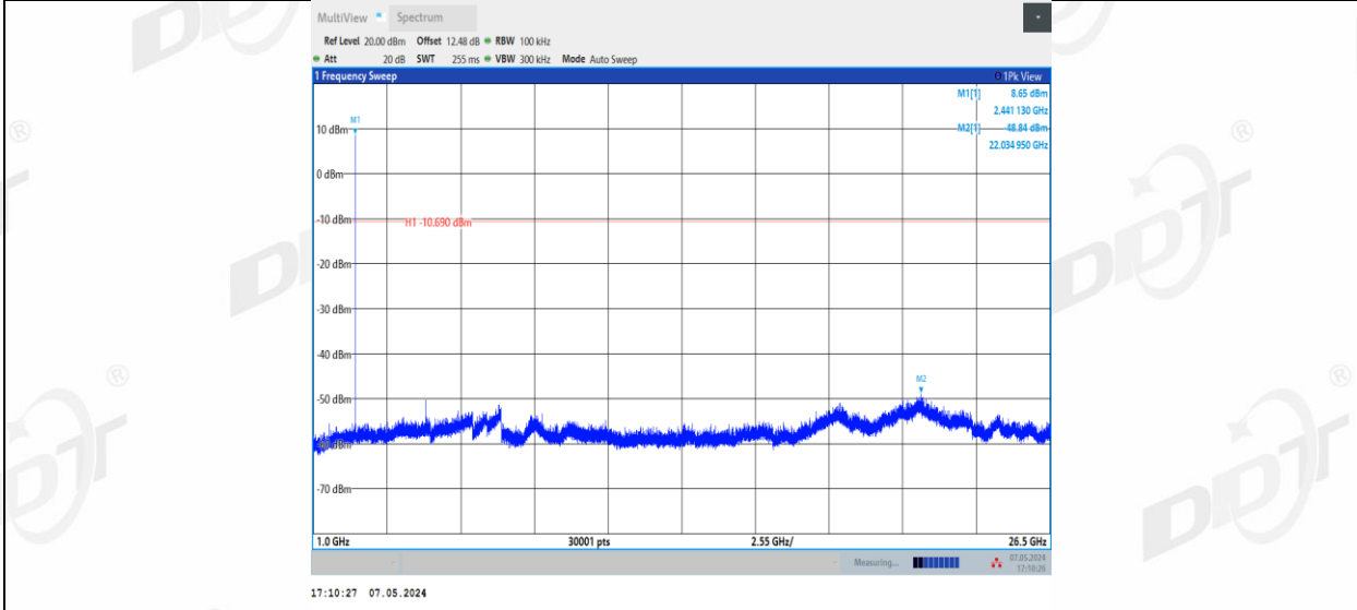
DH5_Ant2_R_2441_0~Reference
