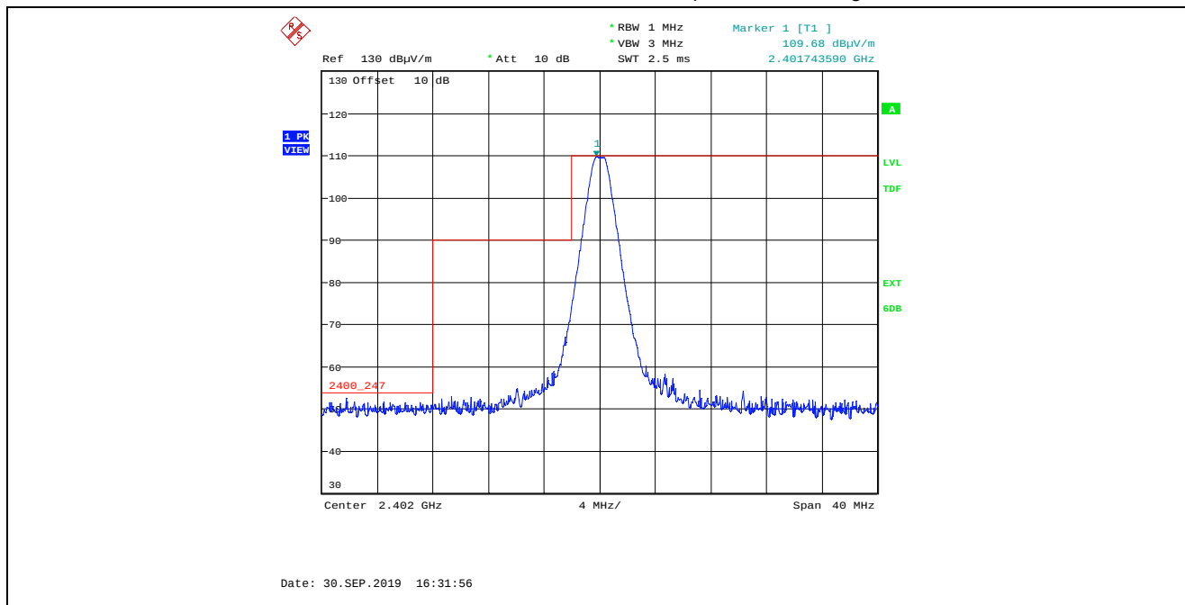
Plot 5.2.4.2.1. Band-Edge Radiated Emissions, Lower Band- edge, Peak Detector Rx Antenna in Vertical Polarization, GFSK Modulation, 1 Mbps, Power Setting 200, Ch 00, 2402 MHz
