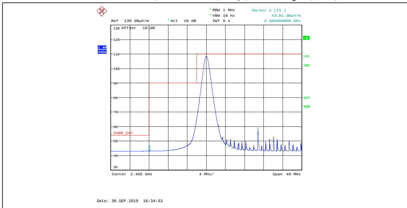
Plot 5.2.4.2.2. Band-Edge Radiated Emissions, Lower Band- edge, Average Detector Rx Antenna in Vertical Polarization, GFSK Modulation, 1 Mbps, Power Setting 200, Ch 00, 2402 MHz
