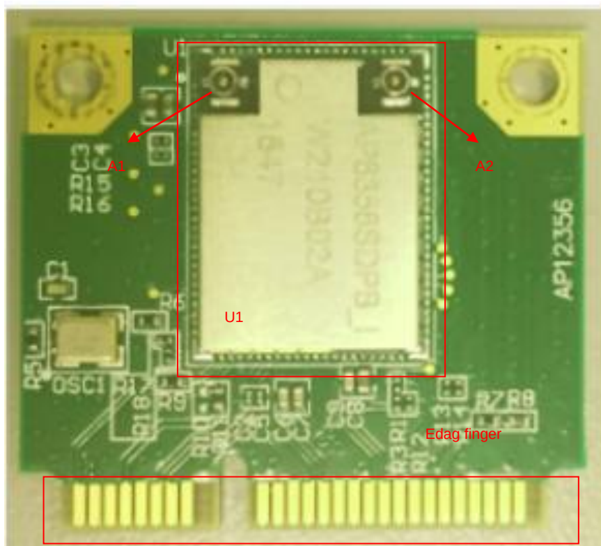
Figure1. Top view of AP6356SDPB_I CB
