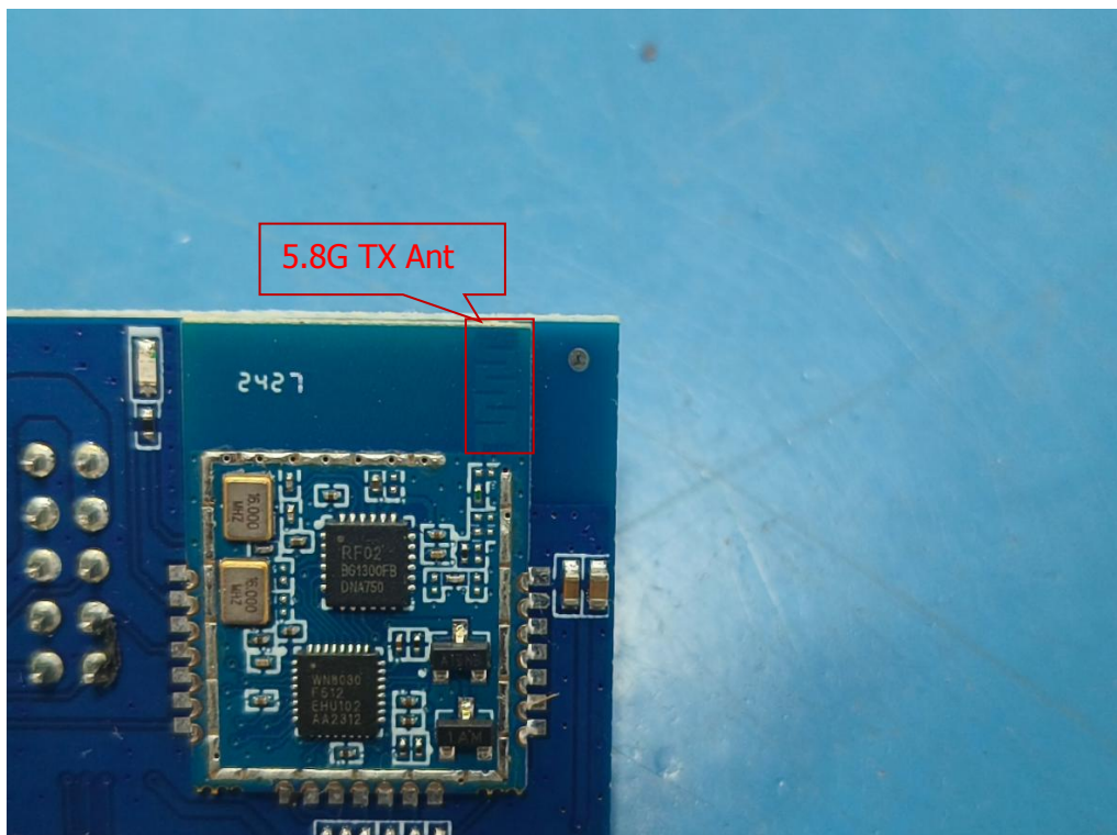
Internal view of unit (Model:A51 PRO)
