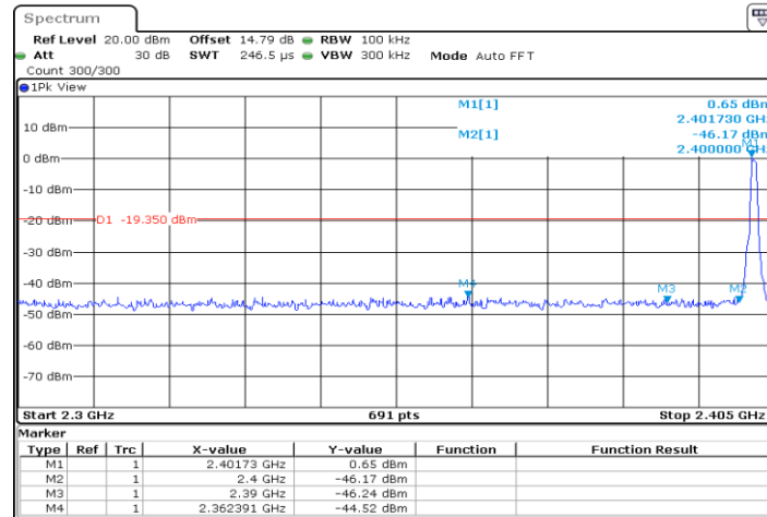
BLE_BT4.0_Ant1_Low_2402
