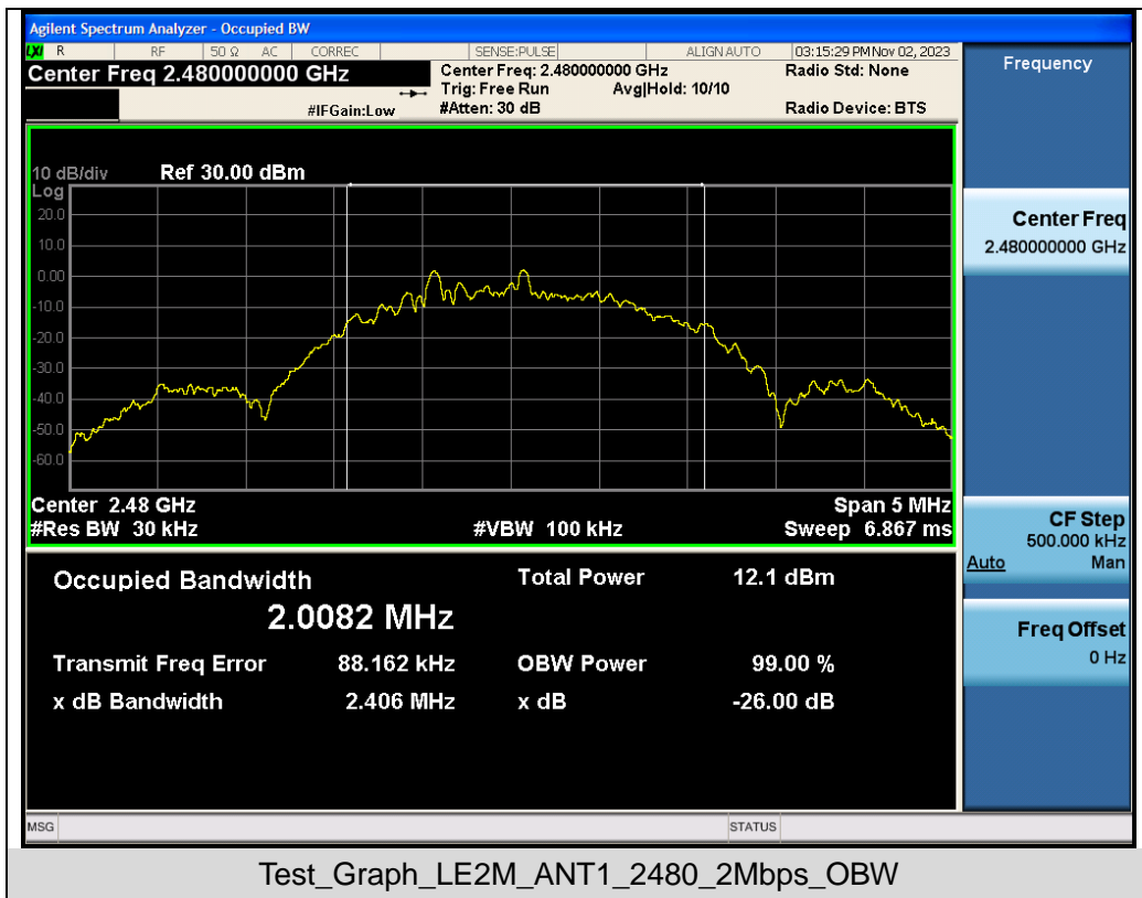
Test_Graph_LE2M_ANT1_2480_2Mbps_OBW Test Graphs of DTS Bandwidth
