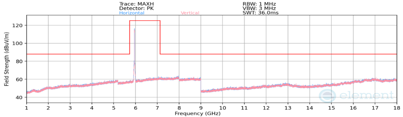
Plot 7-1266. Radiated Spurious Emissions SDM Diversity (802.11ax – Ch. 1)
