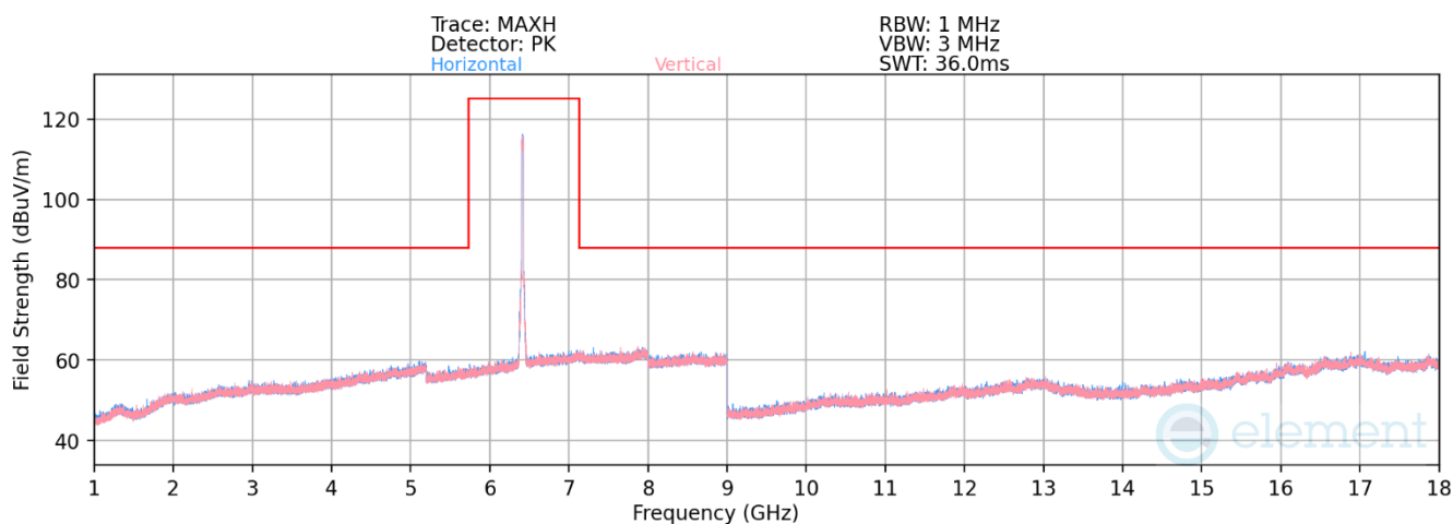
Plot 7-1269. Radiated Spurious Emissions SDM Diversity (802.11ax – Ch. 93)
