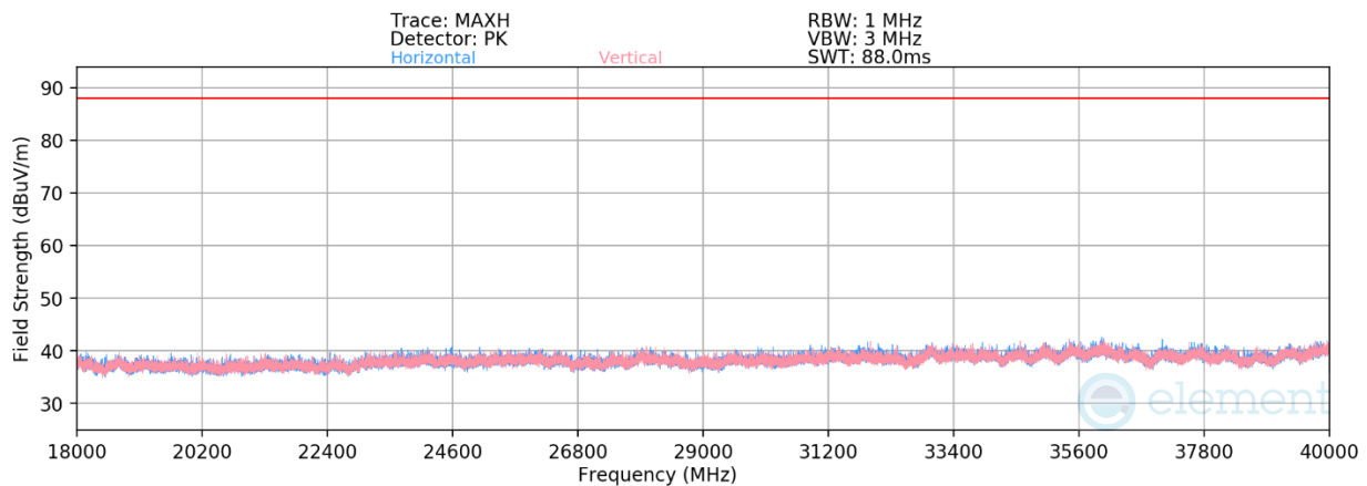
Plot 7-1261. Radiated Spurious Emissions 18-40GHz SDM Primary (802.11ax – Ch. 185)
