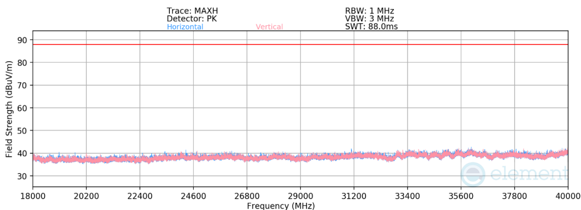
Plot 7-1279. Radiated Spurious Emissions 18-40GHz SDM Diversity (802.11ax – Ch. 189)
