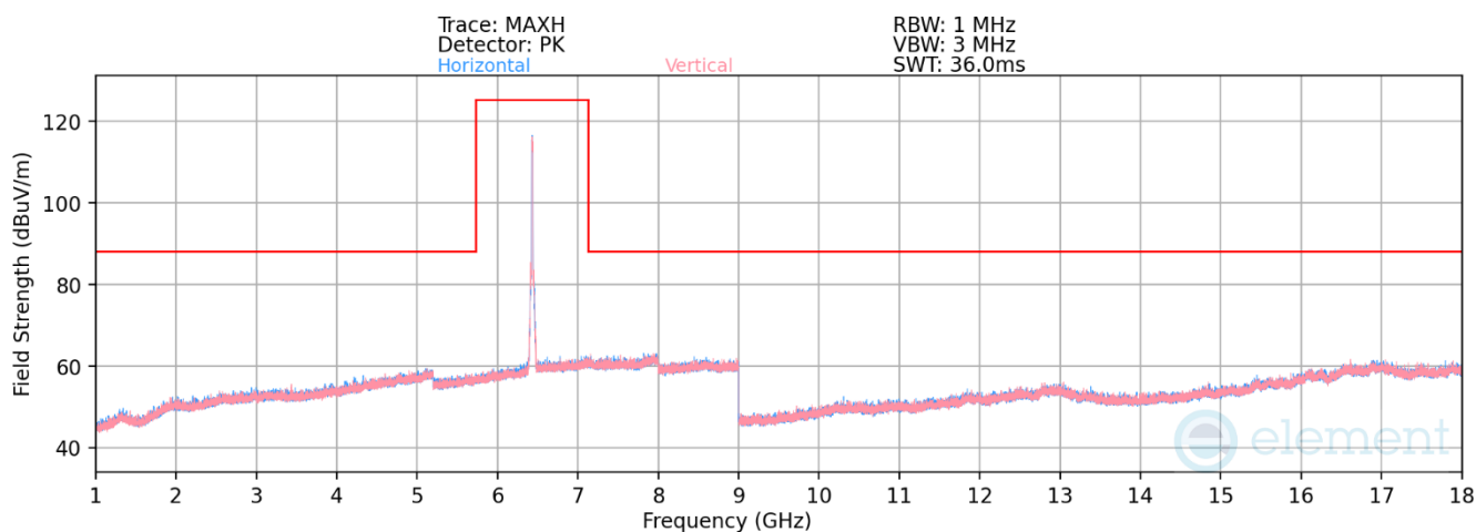
Plot 7-1270. Radiated Spurious Emissions SDM Diversity (802.11ax – Ch. 93)
