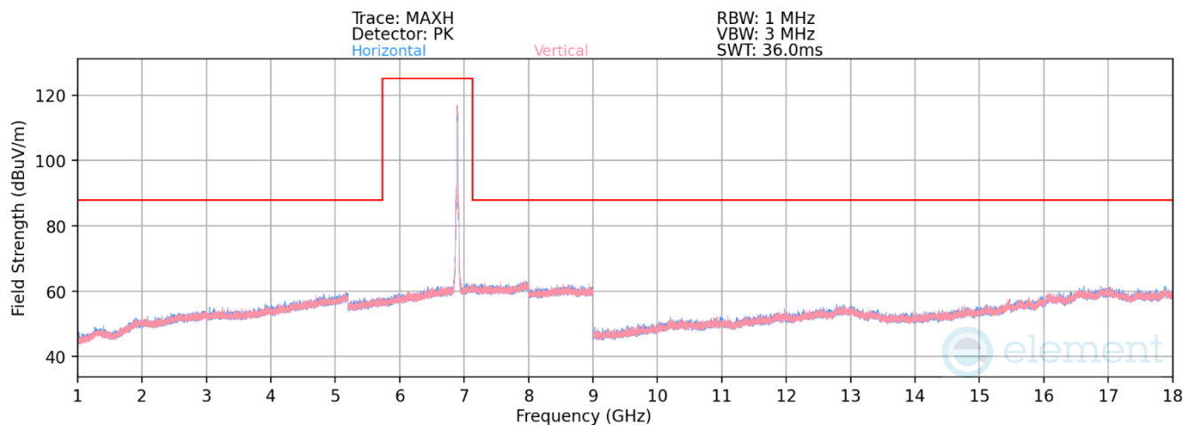
Plot 7-1278. Radiated Spurious Emissions SDM Diversity (802.11ax – Ch. 189)
