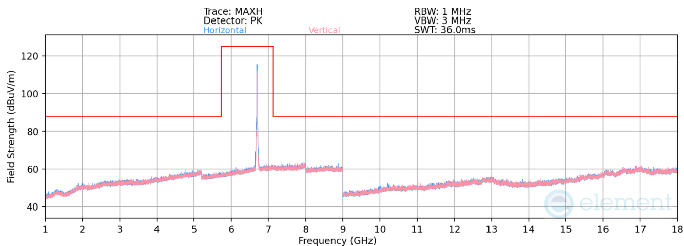
Plot 7-1259. Radiated Spurious Emissions SDM Primary (802.11ax – Ch. 149)
