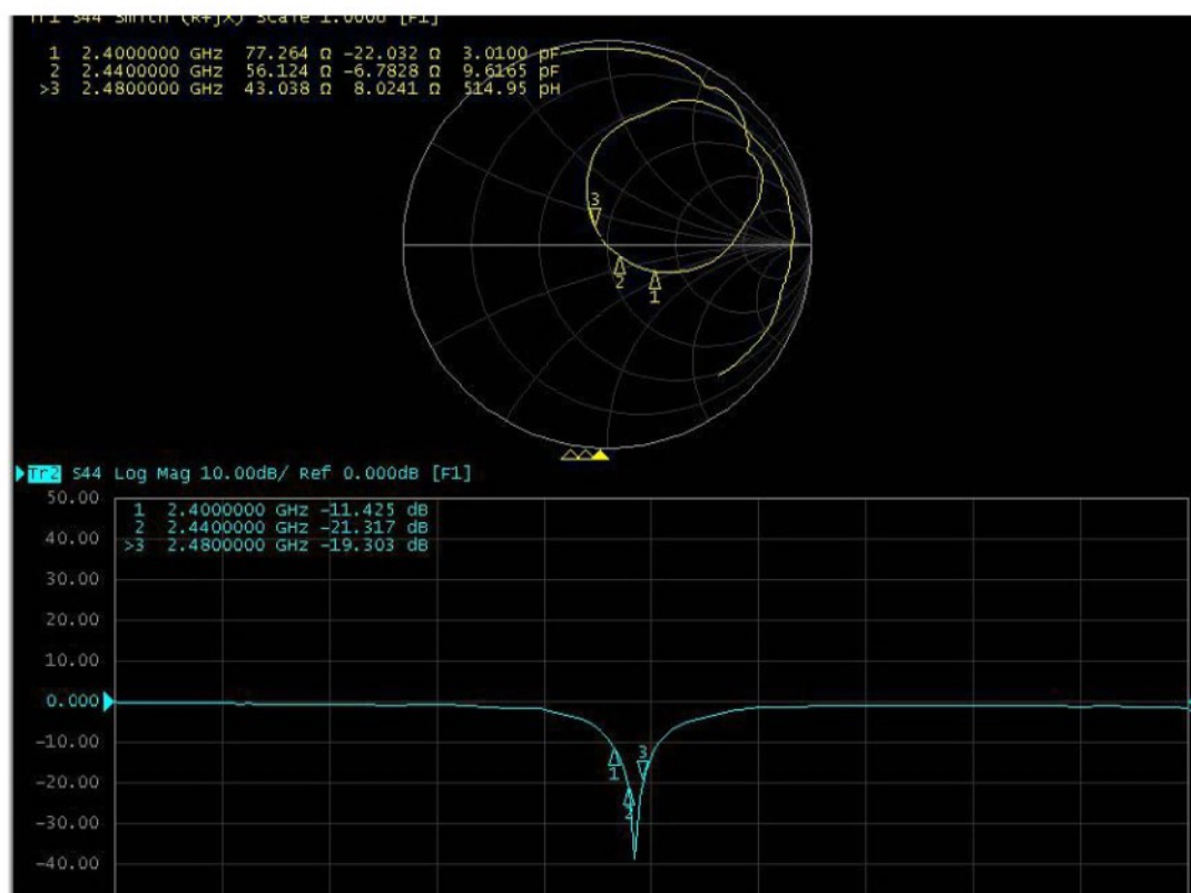
Return Loss
