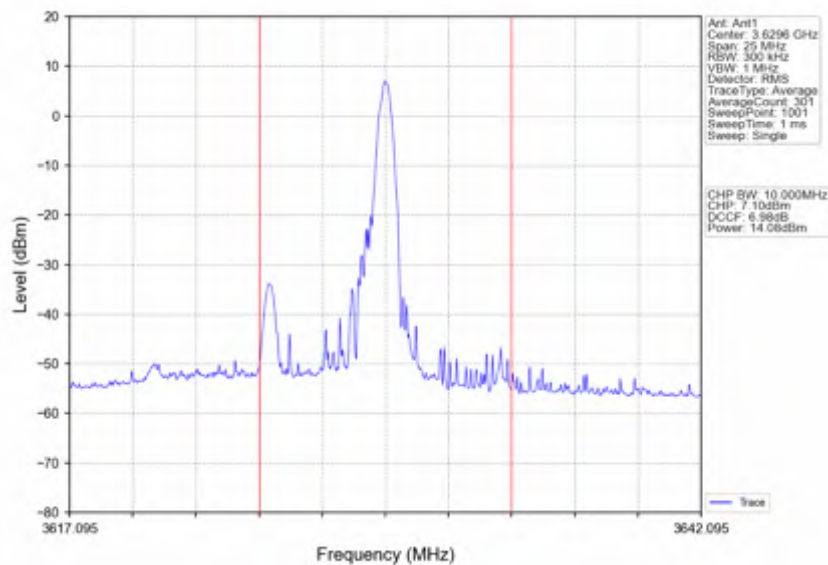
n78d_15kHz_SISO_NTNV_10MHz_CP-OFDM 64 QAM_3625.005MHz_Edge_1RB_Right
