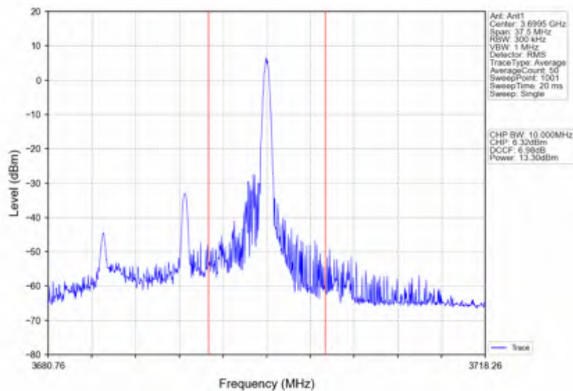
n78d_15kHz_SISO_NTV_15MHz_CP-OFDM QPSK_3692.49MHz_Edge_1RB_Right
