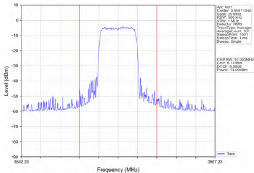
n78d_15kHz_SISO_NTNV_10MHz_DFT-s-OFDM_256_QAM_3555MHz_Inner_Full
