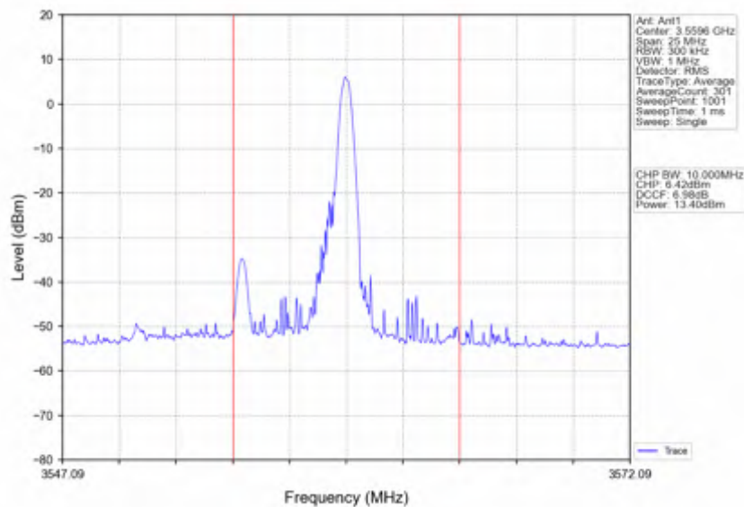
n78d_15kHz_SISO_NTNV_10MHz_CP-OFDM 64 QAM_3555MHz_Edge_1RB_Right
