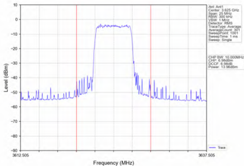
n78d_15kHz_SISO_NTNV_10MHz_CP-OFDM 256 QAM_3625.005MHz_Inner_Full
