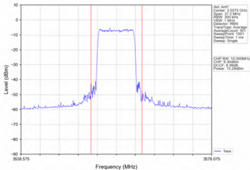
n78d_15kHz_SISO_NTNV_15MHz_CP-OFDM_16_QAM_3557.505MHz_Inner_Full
