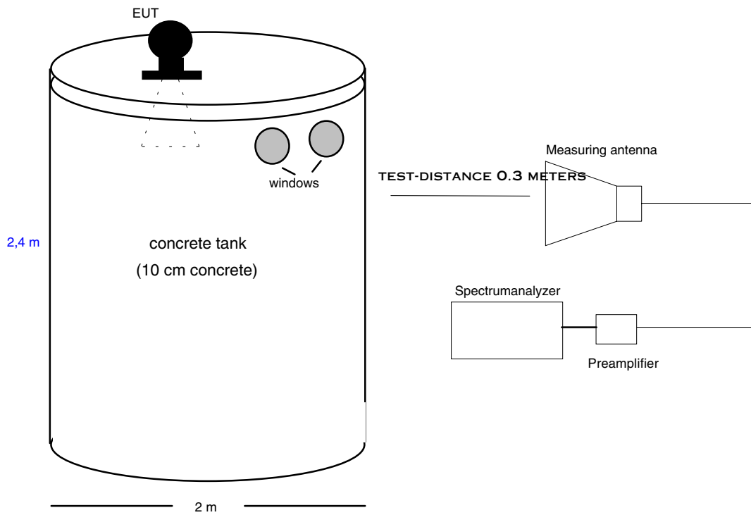
fig.2 application in a concrete tank
