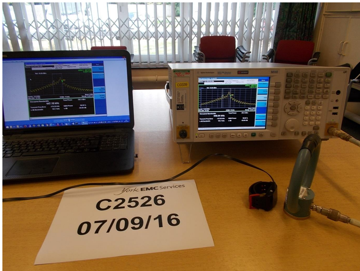
Occupied Bandwidth Set IUp
