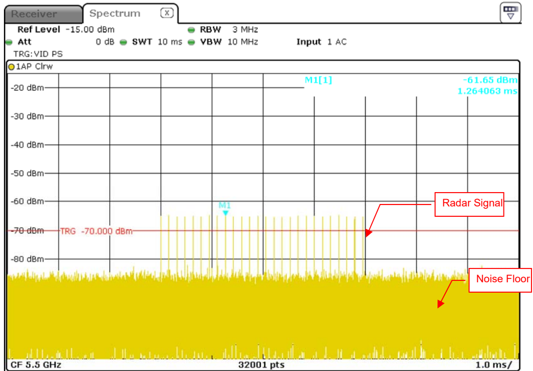
Radar Signal 2
