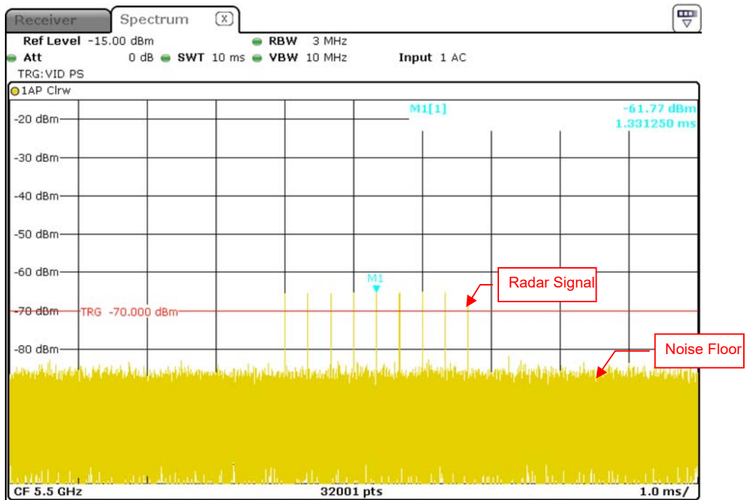
Radar Signal 6
