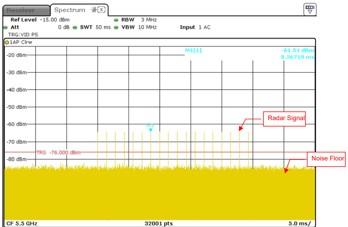
Radar Signal 0
