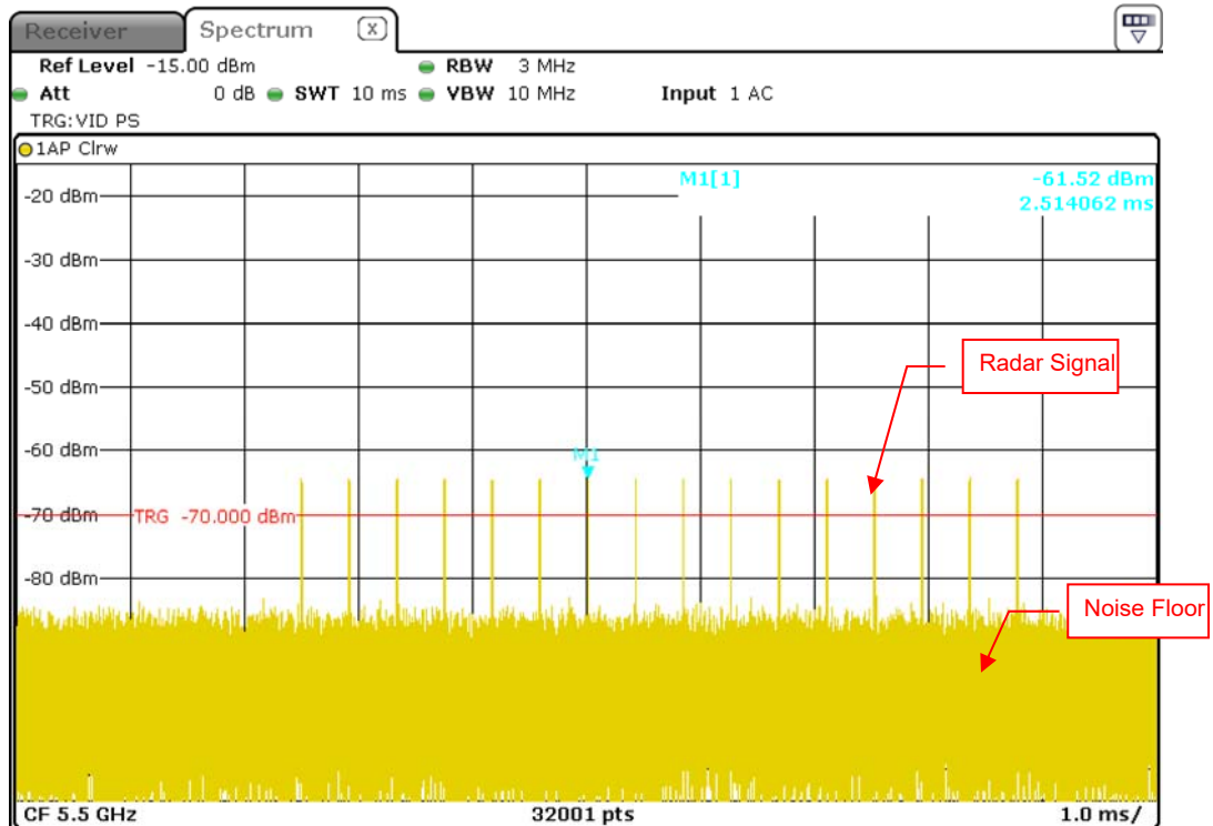
Radar Signal 3
