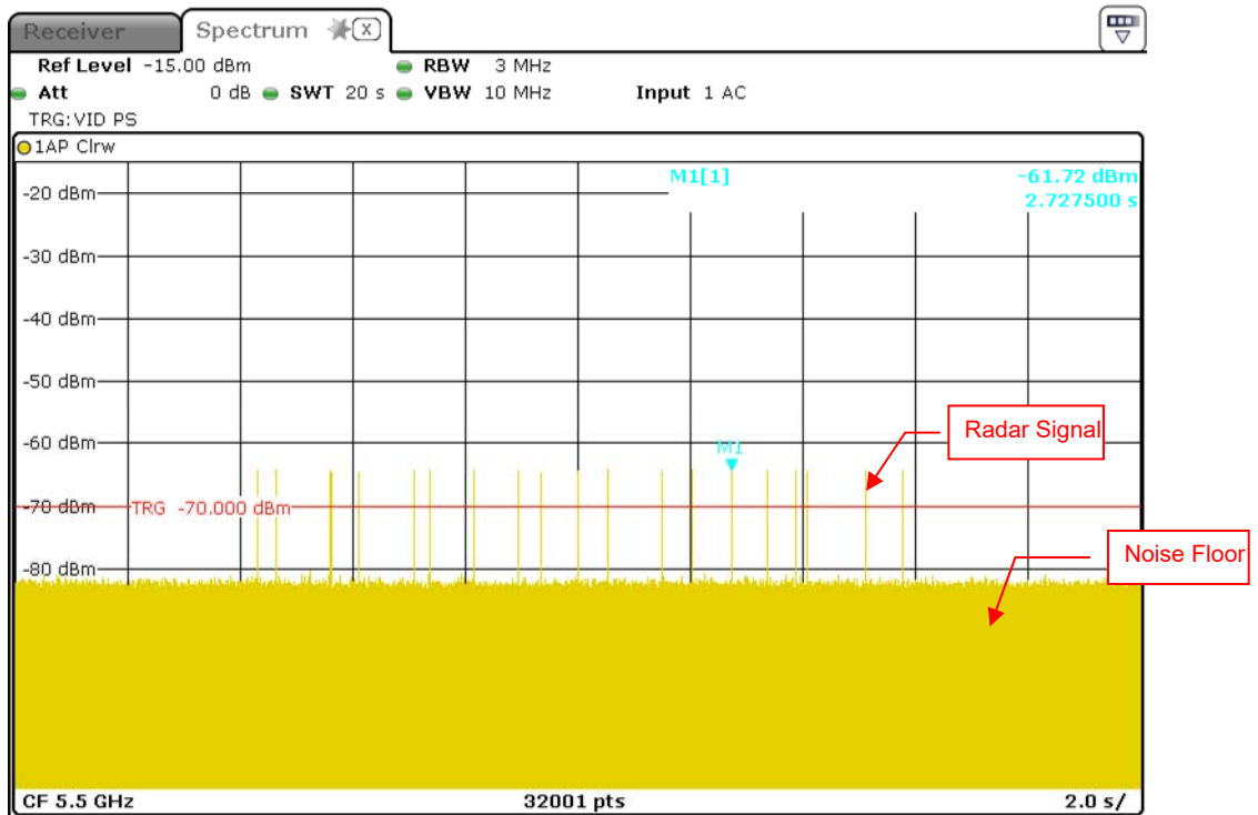
Radar Signal 5
