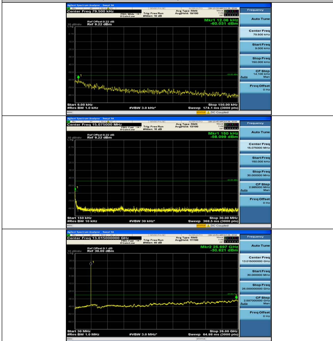
(Channel Bandwidth 15 MHz)_LCH_QPSK_1RB#0
