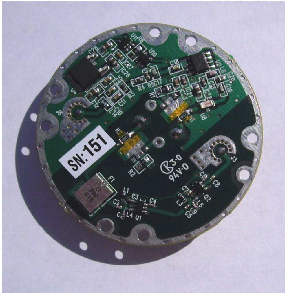
Figure 7 ODU Antenna PCB Bottom
