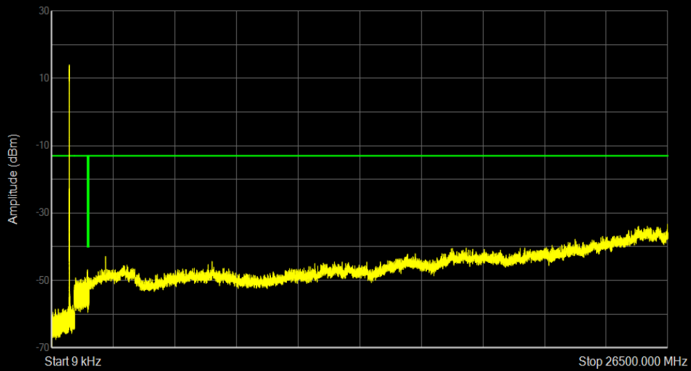
Band13 16QAM BW=5MHz Channel=23205 RB Size=25 Position=#0
