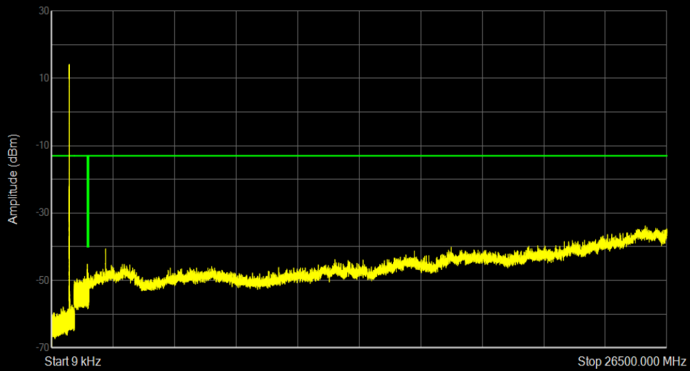
Band13 16QAM BW=5MHz Channel=23230 RB Size=25 Position=#0
