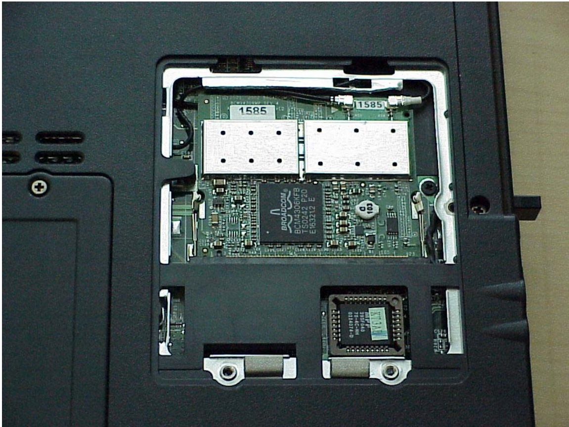
Photo 3. EUT in PC
