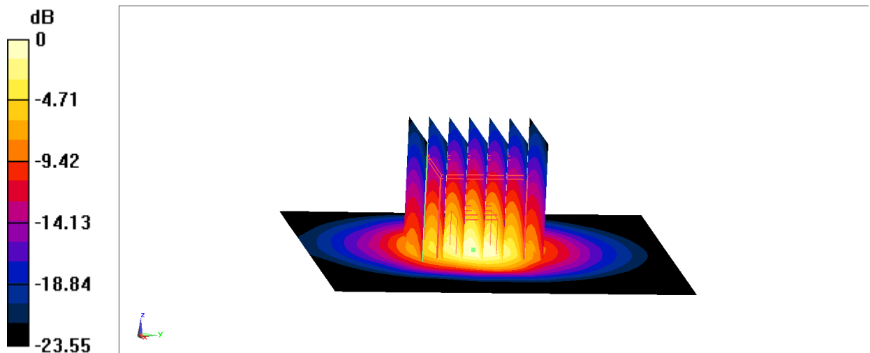
Fig.B.6 validation 2600 MHz 250mW
