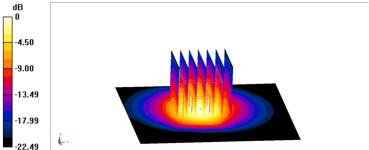
Fig.B.5 validation 2450 MHz 250mW
