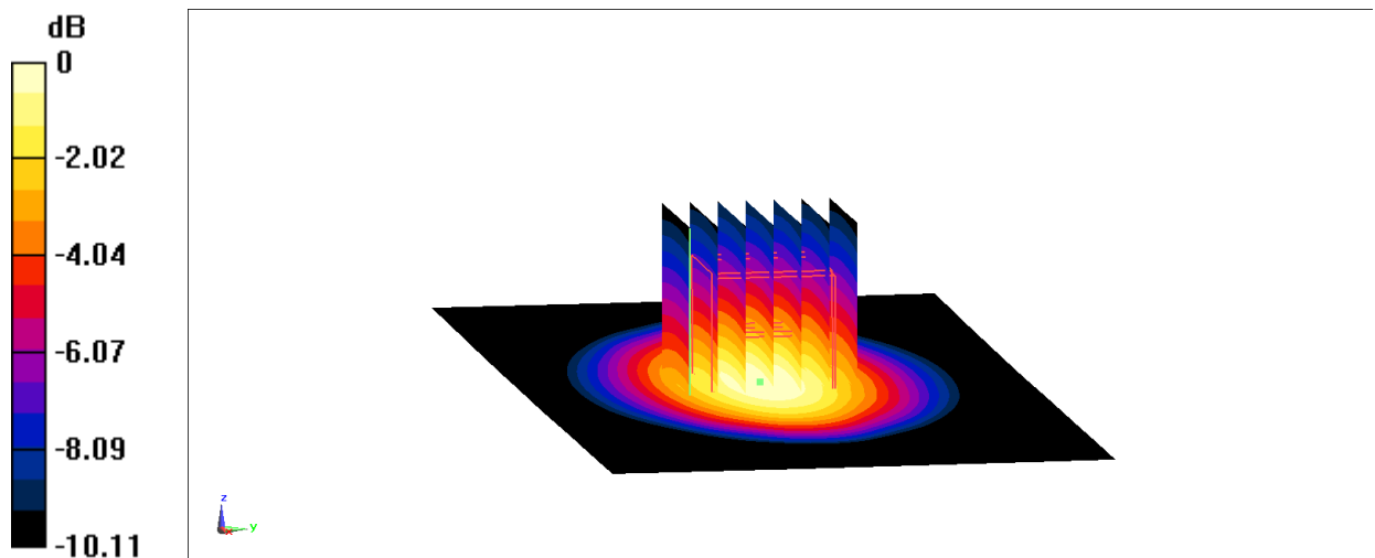
Fig.B.2 validation 835 MHz 250mW
