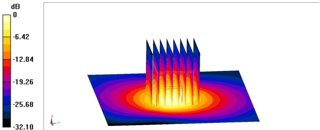
Fig.B.7 validation 3500 MHz 100mW
