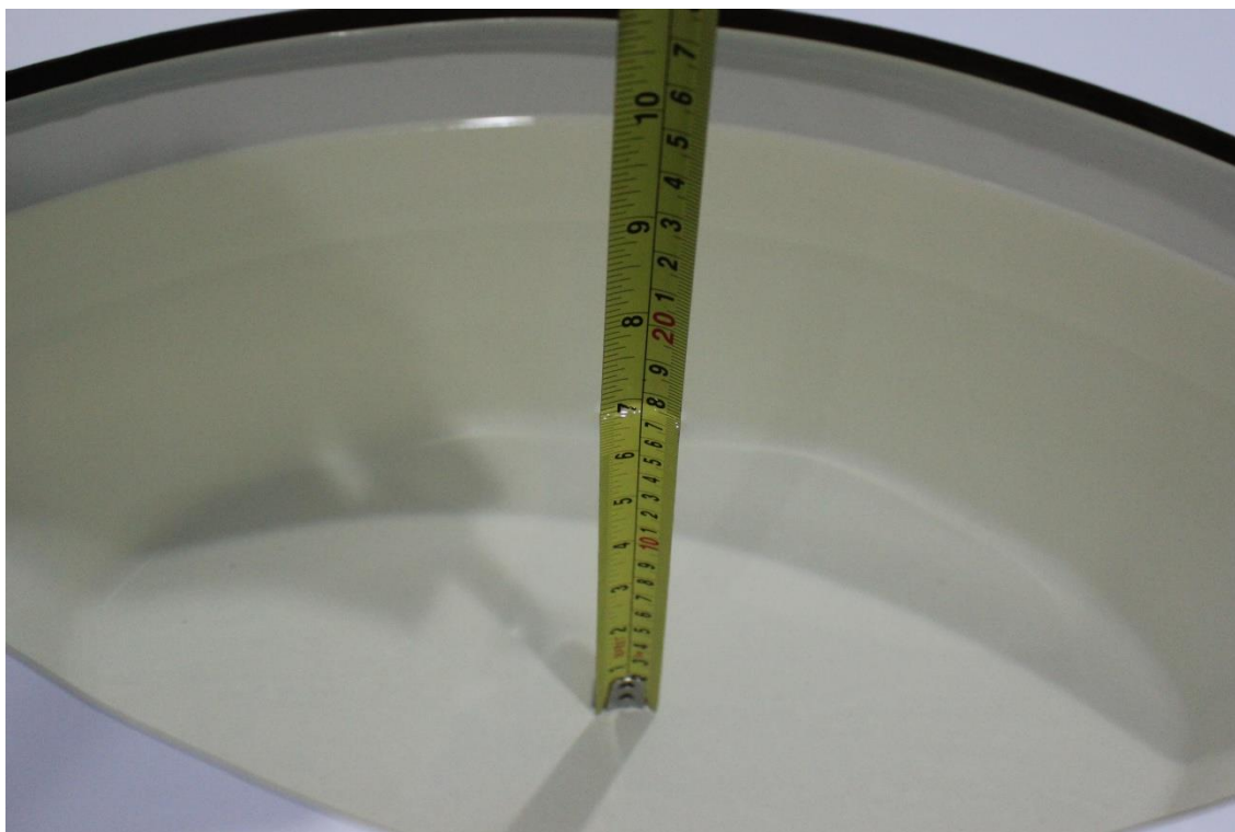
Picture 8-9 Liquid depth in the Head Phantom (5GHz)
