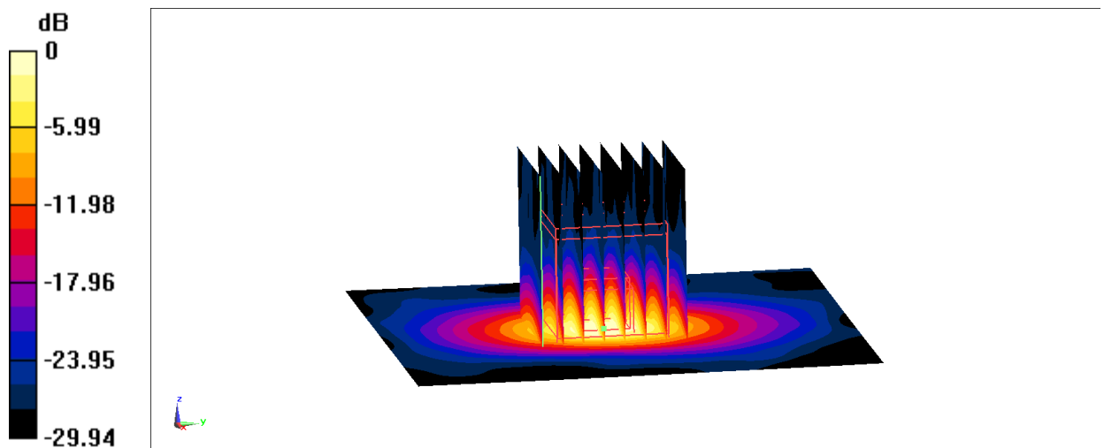
Fig.B.12 validation 5750 MHz 100mW
