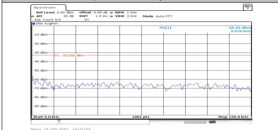
Band4-1.4MHz-16QAM-19957-1RB#0-Range1:0.009~0.15MHz-PASS
