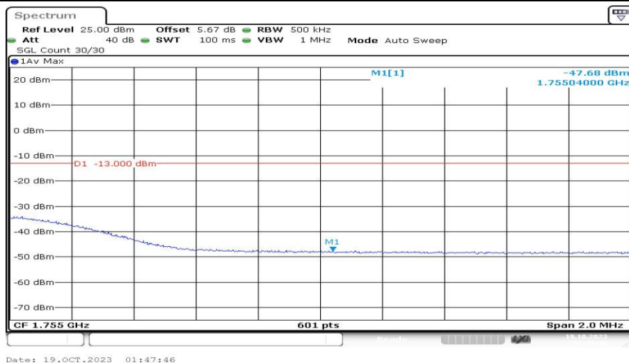
Band4-20MHz-16QAM-20300-1RB#0-PASS
