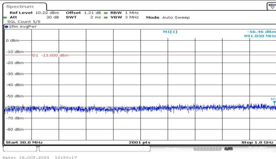
Band4-5MHz-QPSK-19975-1RB#0-Range3:30~1000MHz-PASS
