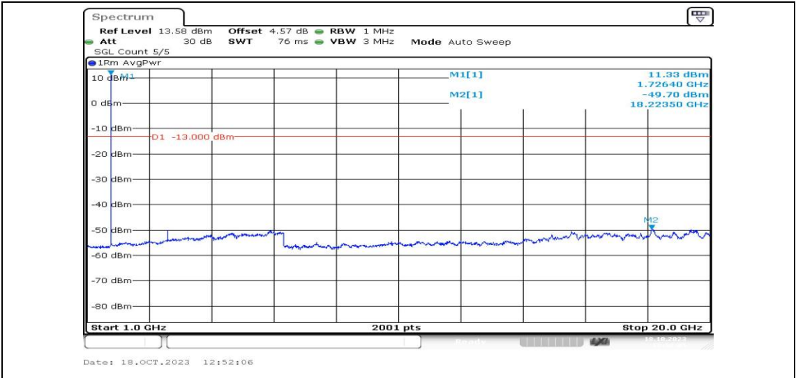
Band4-5MHz-QPSK-20175-1RB#0-Range4:1000~20000MHz-PASS
