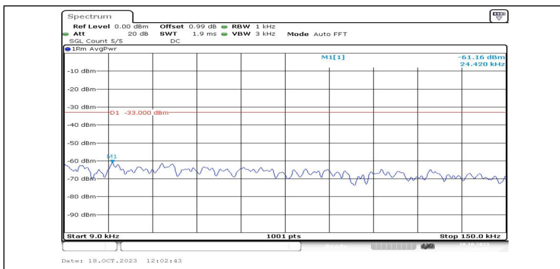
Band4-1.4MHz-QPSK-20175-1RB#0-Range1:0.009~0.15MHz-PASS
