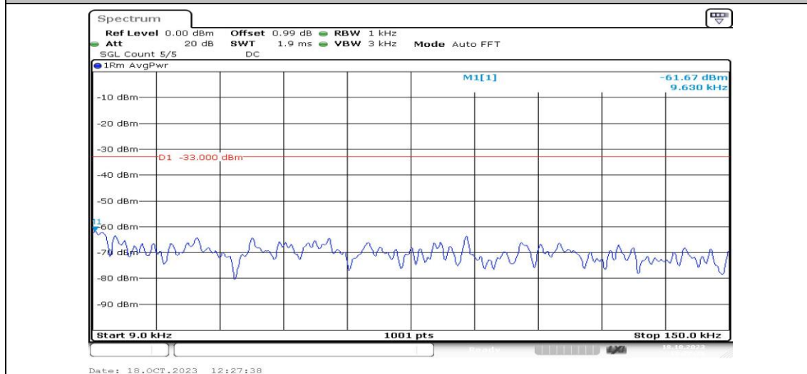
Band4-3MHz-16QAM-20175-1RB#0-Range1:0.009~0.15MHz-PASS
