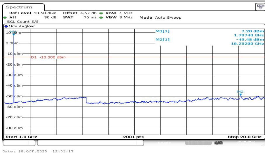
Band4-5MHz-16QAM-19975-1RB#0-Range4:1000~20000MHz-PASS
