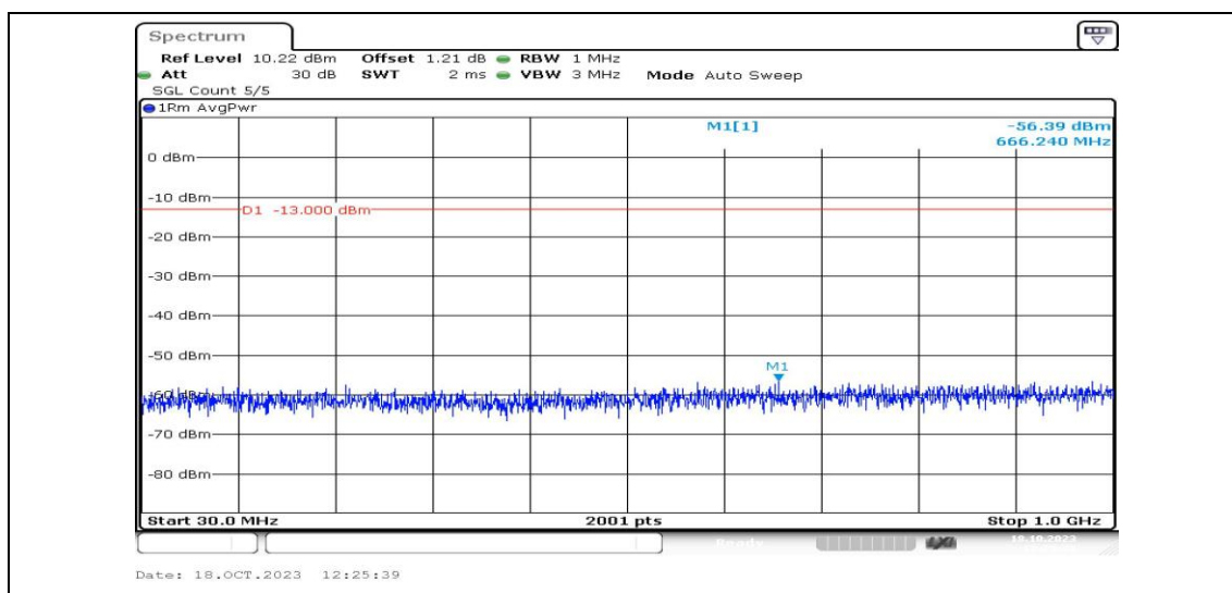
Band4-3MHz-QPSK-19965-1RB#0-Range3:30~1000MHz-PASS
