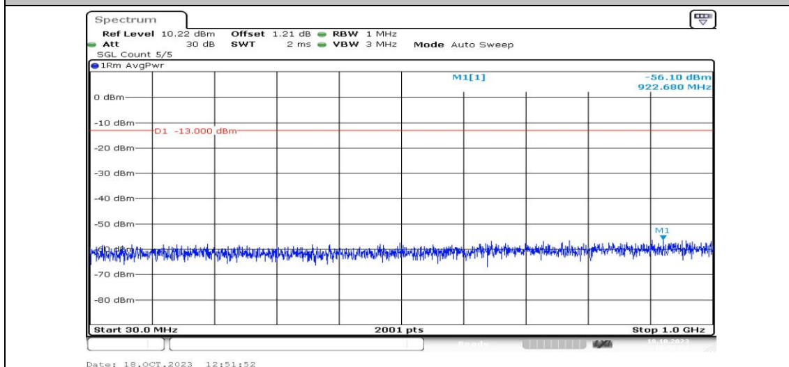
Band4-5MHz-QPSK-20175-1RB#0-Range3:30~1000MHz-PASS
