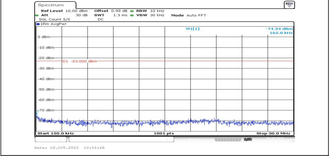
Band4-5MHz-16QAM-20175-1RB#0-Range2:0.15~30MHz-PASS
