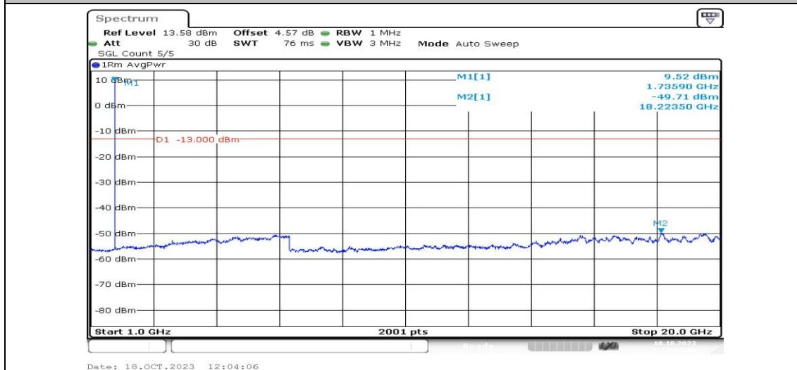
Band4-1.4MHz-16QAM-20175-1RB#0-Range4:1000~20000MHz-PASS
