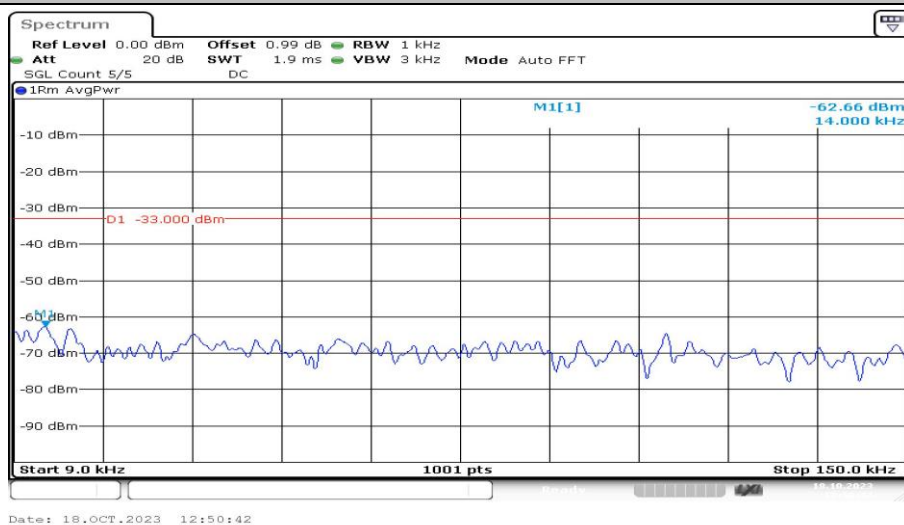
Band4-5MHz-16QAM-19975-1RB#0-Range1:0.009~0.15MHz-PASS
