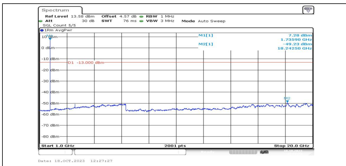
Band4-3MHz-QPSK-20175-1RB#0-Range4:1000~20000MHz-PASS
