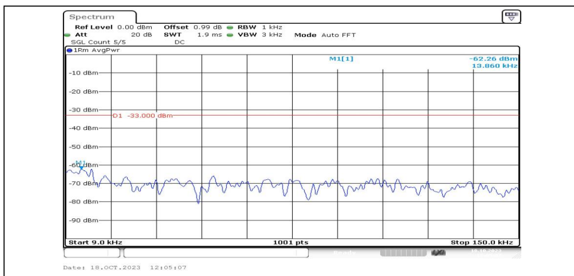
Band4-1.4MHz-16QAM-20393-1RB#0-Range1:0.009~0.15MHz-PASS
