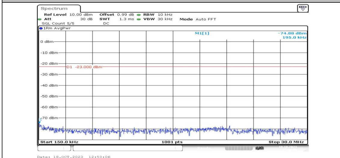
Band4-5MHz-QPSK-19975-1RB#0-Range2:0.15~30MHz-PASS
