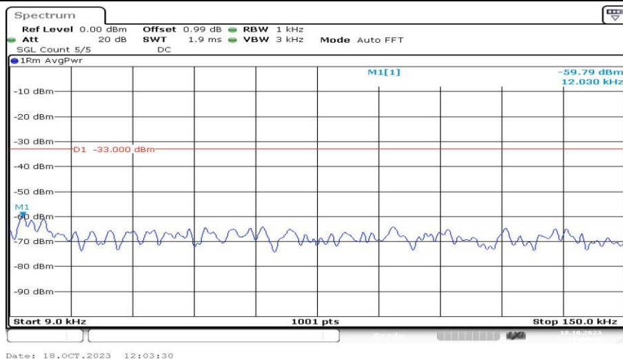
Band4-1.4MHz-16QAM-20175-1RB#0-Range1:0.009~0.15MHz-PASS
