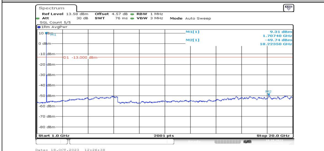
Band4-3MHz-16QAM-19965-1RB#0-Range4:1000~20000MHz-PASS
