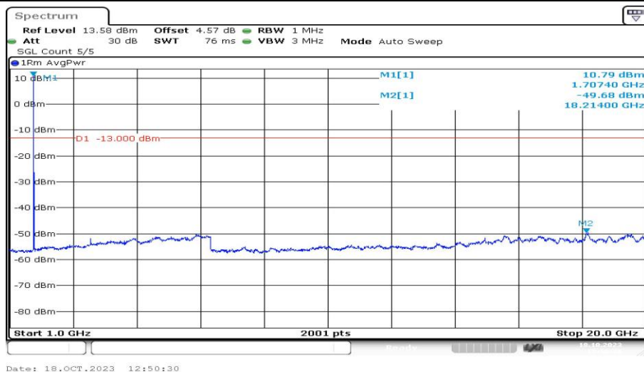
Band4-5MHz-QPSK-19975-1RB#0-Range4:1000~20000MHz-PASS
