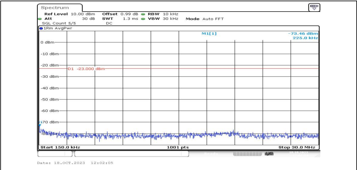
Band4-1.4MHz-16QAM-19957-1RB#0-Range2:0.15~30MHz-PASS
