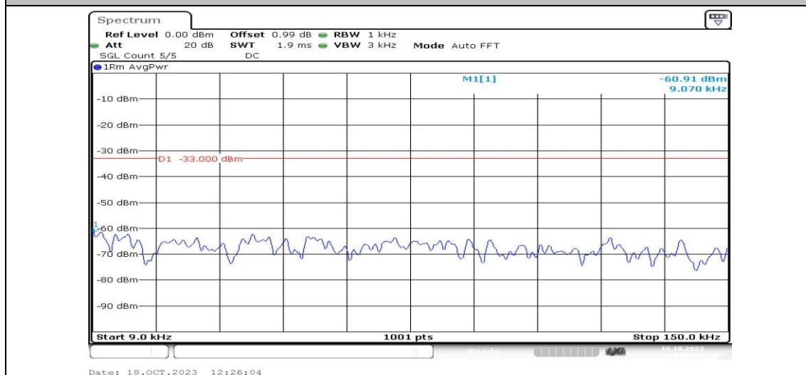
Band4-3MHz-16QAM-19965-1RB#0-Range1:0.009~0.15MHz-PASS
