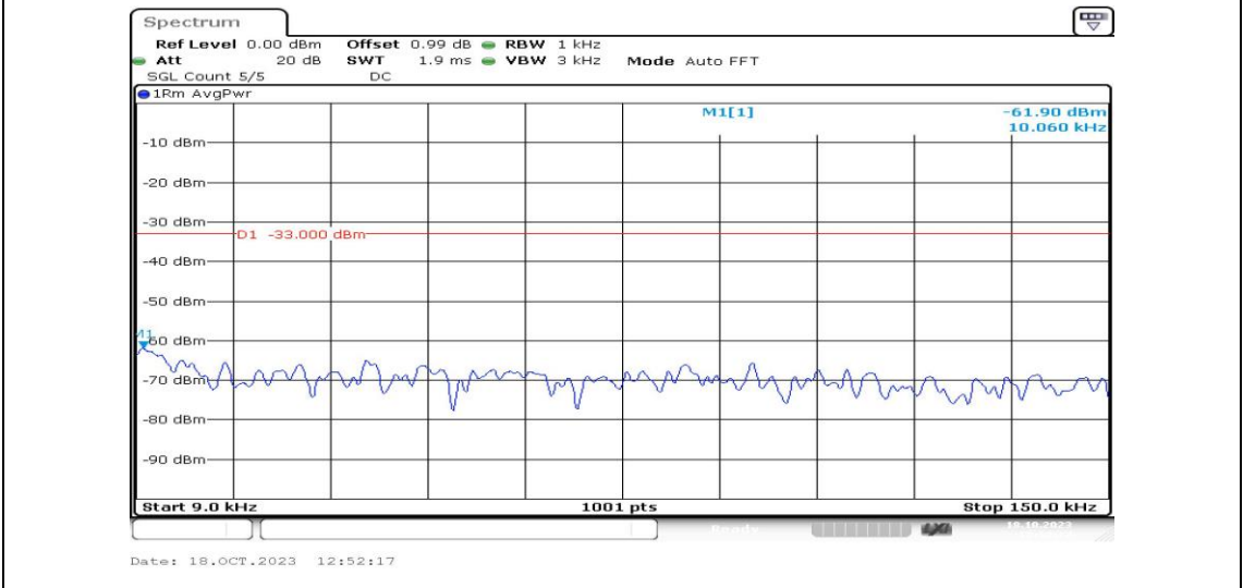
Band4-5MHz-16QAM-20175-1RB#0-Range1:0.009~0.15MHz-PASS
