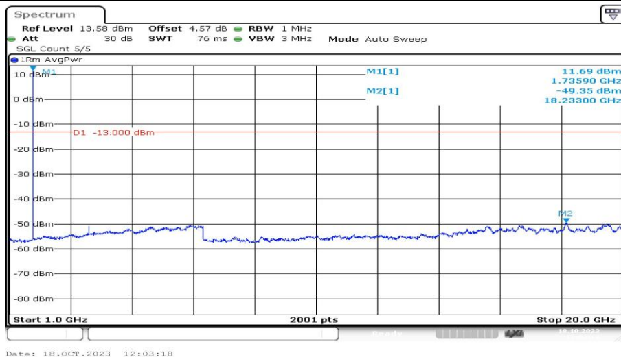
Band4-1.4MHz-QPSK-20175-1RB#0-Range4:1000~20000MHz-PASS
