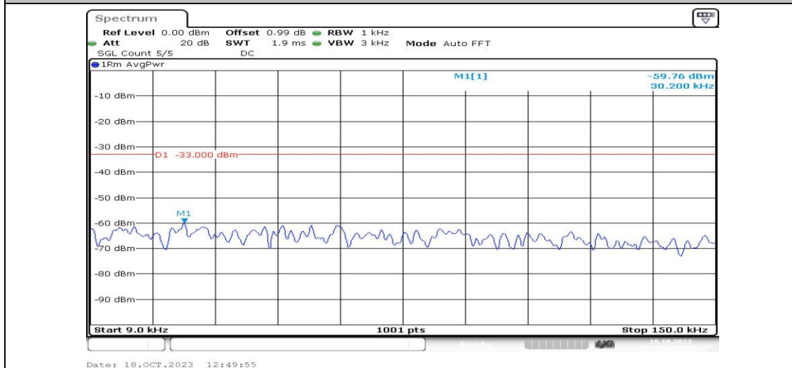
Band4-5MHz-QPSK-19975-1RB#0-Range1:0.009~0.15MHz-PASS
