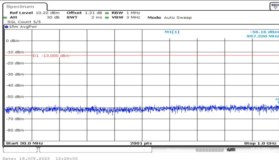
Band4-3MHz-16QAM-20175-1RB#0-Range3:30~1000MHz-PASS
