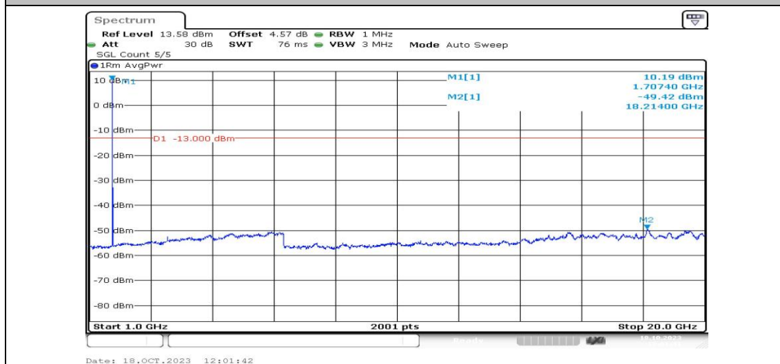
Band4-1.4MHz-QPSK-19957-1RB#0-Range4:1000~20000MHz-PASS
