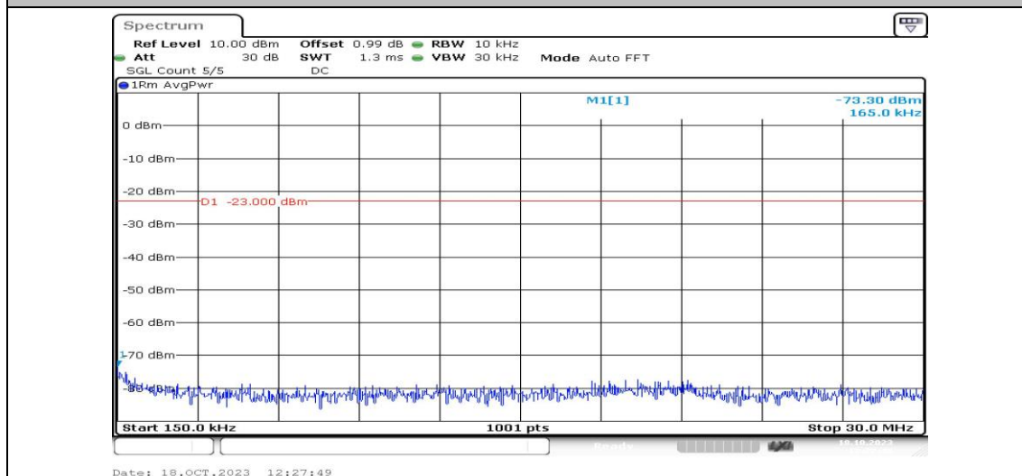
Band4-3MHz-16QAM-20175-1RB#0-Range2:0.15~30MHz-PASS
