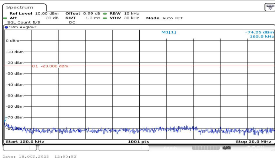
Band4-5MHz-16QAM-19975-1RB#0-Range2:0.15~30MHz-PASS
