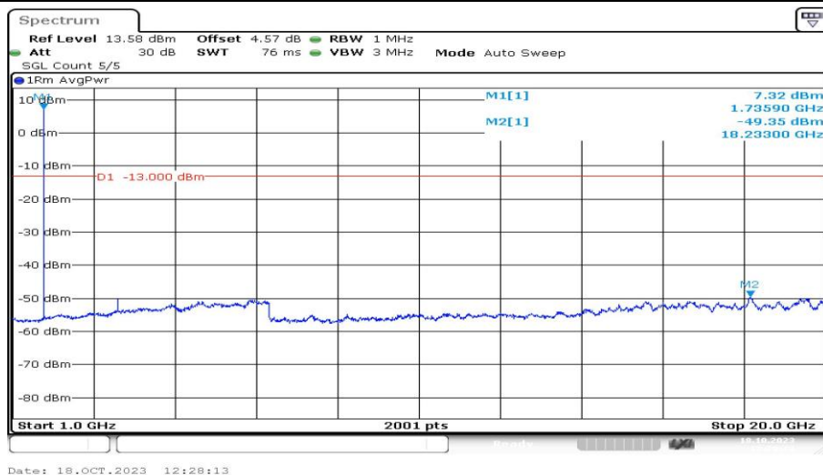
Band4-3MHz-16QAM-20175-1RB#0-Range4:1000~20000MHz-PASS
