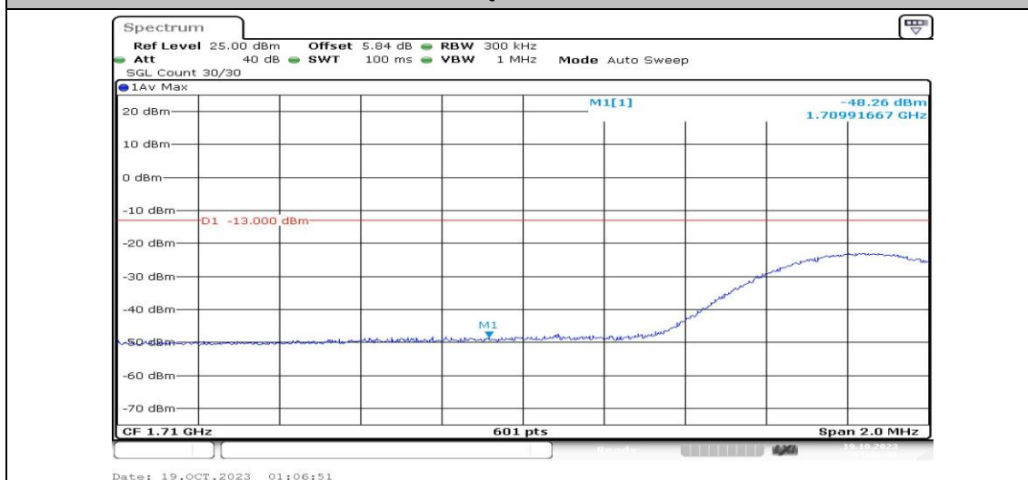
Band4-15MHz-16QAM-20025-1RB#74-PASS
