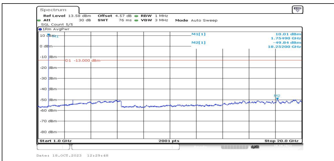
Band4-3MHz-16QAM-20385-1RB#0-Range4:1000~20000MHz-PASS
