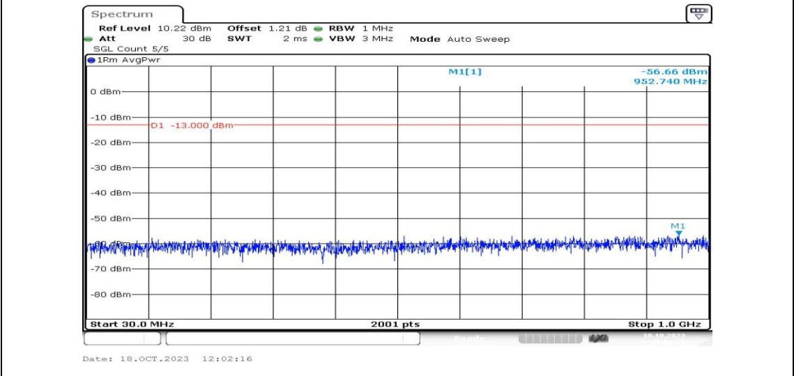
Band4-1.4MHz-16QAM-19957-1RB#0-Range3:30~1000MHz-PASS
