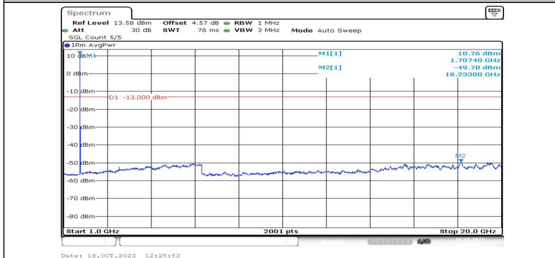
Band4-3MHz-QPSK-19965-1RB#0-Range4:1000~20000MHz-PASS
