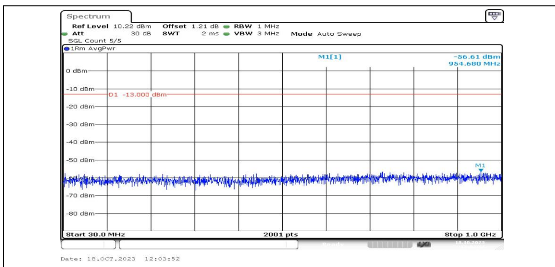
Band4-1.4MHz-16QAM-20175-1RB#0-Range3:30~1000MHz-PASS
