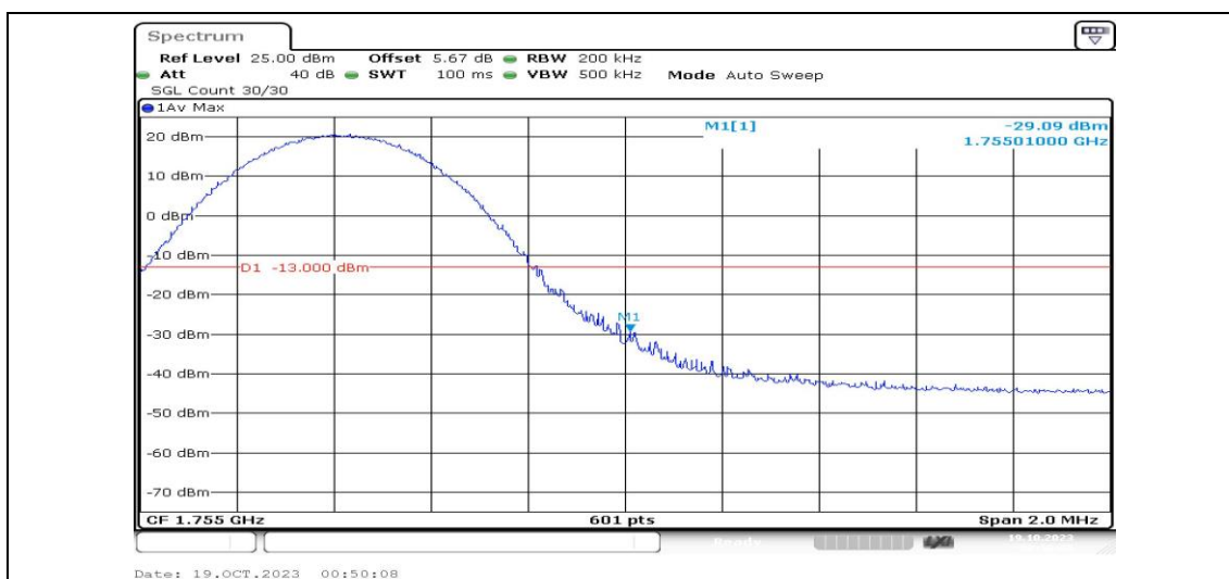
Band4-10MHz-16QAM-20350-1RB#49-PASS
