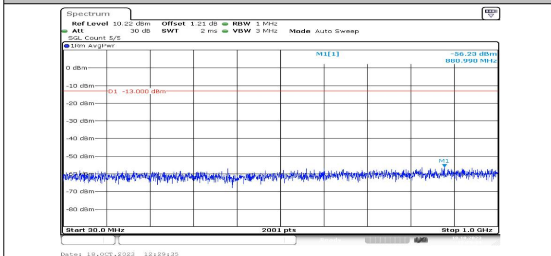
Band4-3MHz-16QAM-20385-1RB#0-Range3:30~1000MHz-PASS
