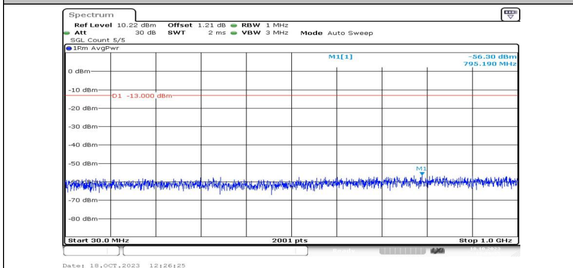
Band4-3MHz-16QAM-19965-1RB#0-Range3:30~1000MHz-PASS
