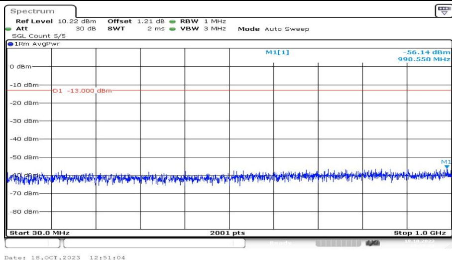
Band4-5MHz-16QAM-19975-1RB#0-Range3:30~1000MHz-PASS
