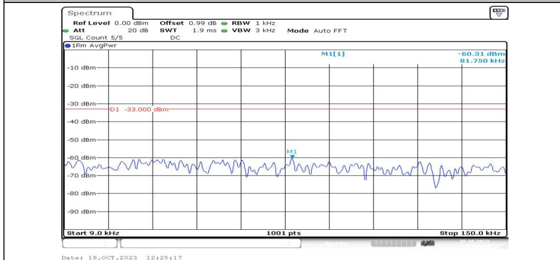
Band4-3MHz-QPSK-19965-1RB#0-Range1:0.009~0.15MHz-PASS
