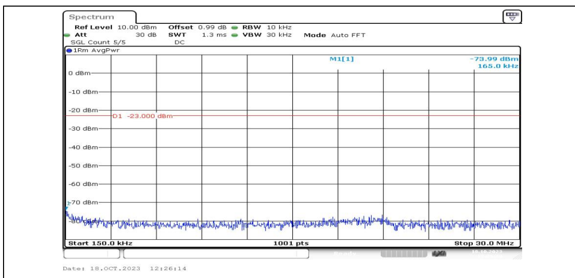
Band4-3MHz-16QAM-19965-1RB#0-Range2:0.15~30MHz-PASS
