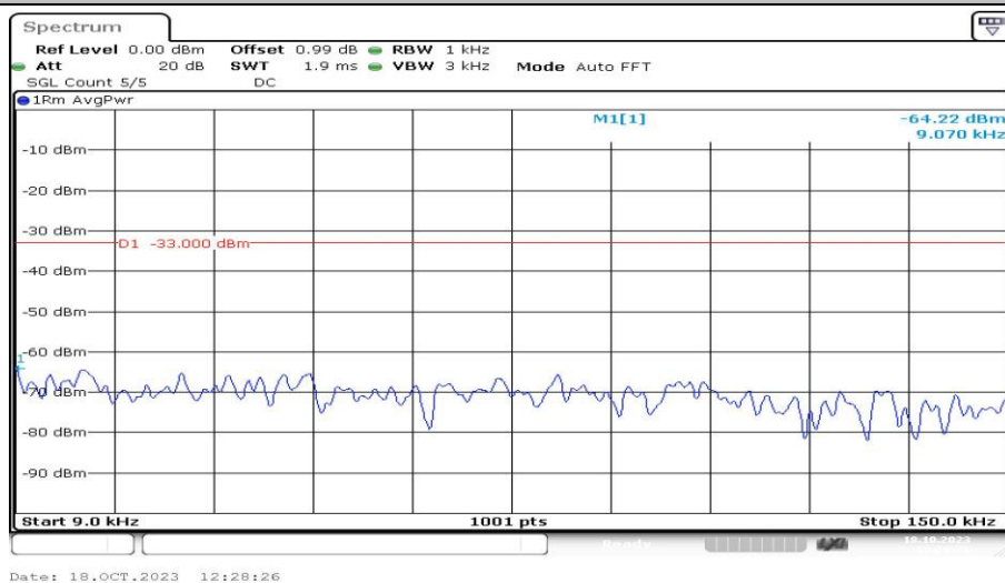
Band4-3MHz-QPSK-20385-1RB#0-Range1:0.009~0.15MHz-PASS
