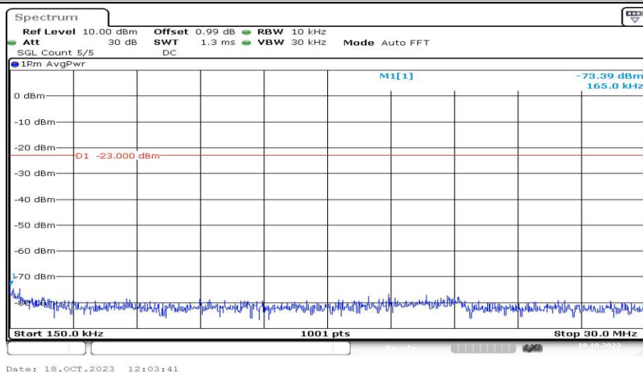
Band4-1.4MHz-16QAM-20175-1RB#0-Range2:0.15~30MHz-PASS
