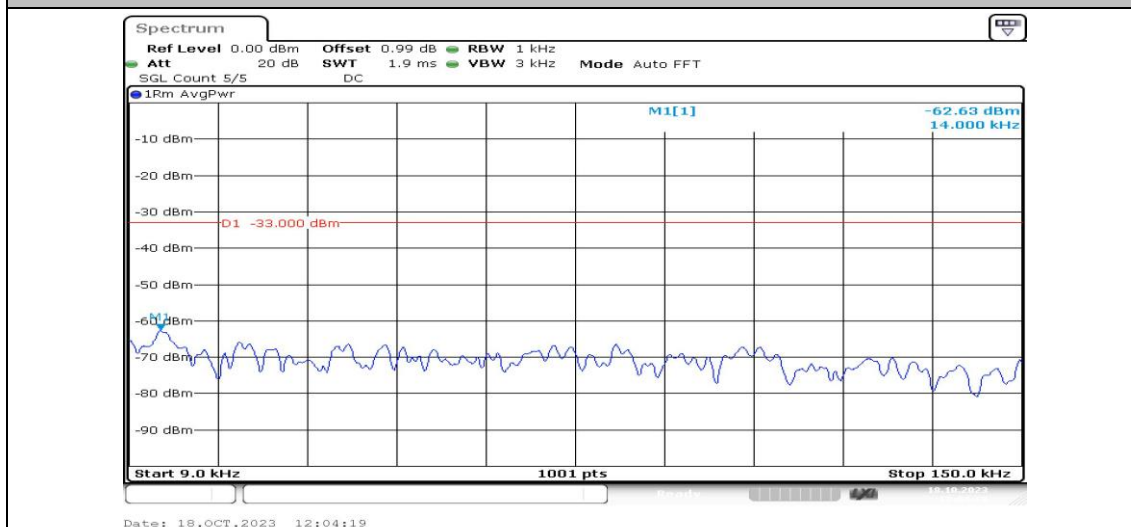
Band4-1.4MHz-QPSK-20393-1RB#0-Range1:0.009~0.15MHz-PASS
