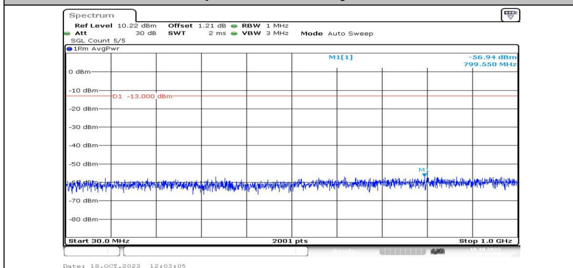
Band4-1.4MHz-QPSK-20175-1RB#0-Range3:30~1000MHz-PASS
