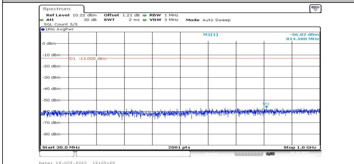
Band4-1.4MHz-16QAM-20393-1RB#0-Range3:30~1000MHz-PASS
