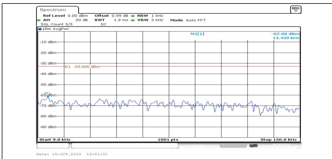
Band4-5MHz-QPSK-20175-1RB#0-Range1:0.009~0.15MHz-PASS
