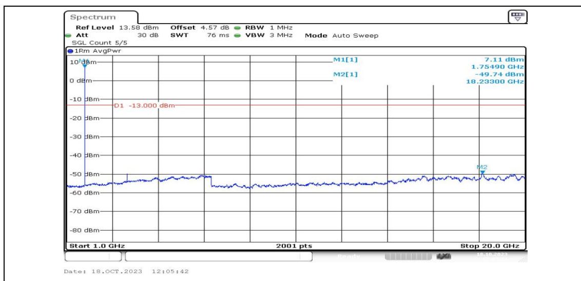
Band4-1.4MHz-16QAM-20393-1RB#0-Range4:1000~20000MHz-PASS
