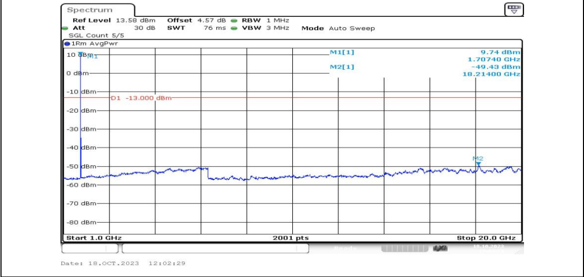
Band4-1.4MHz-16QAM-19957-1RB#0-Range4:1000~20000MHz-PASS
