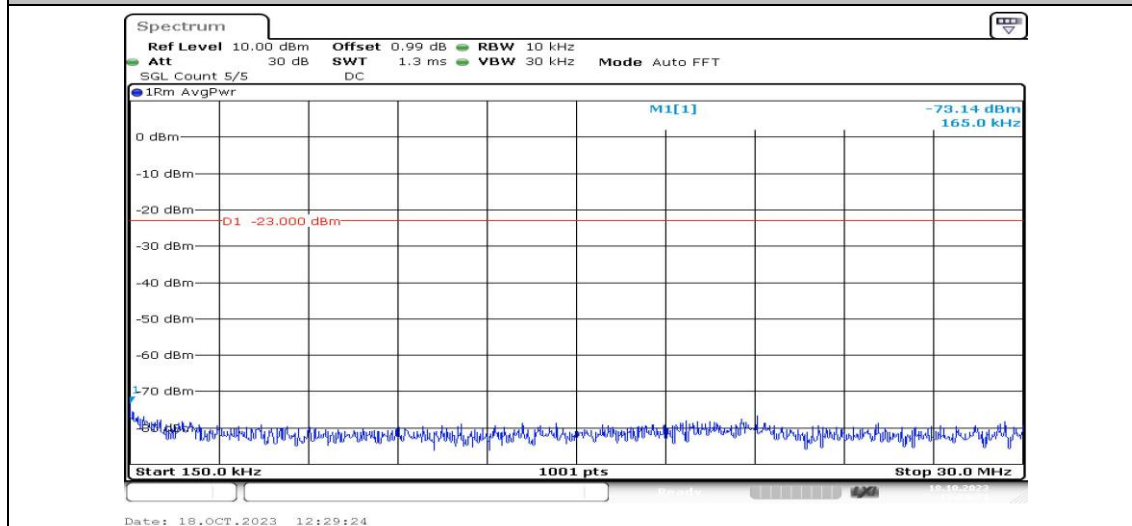
Band4-3MHz-16QAM-20385-1RB#0-Range2:0.15~30MHz-PASS
