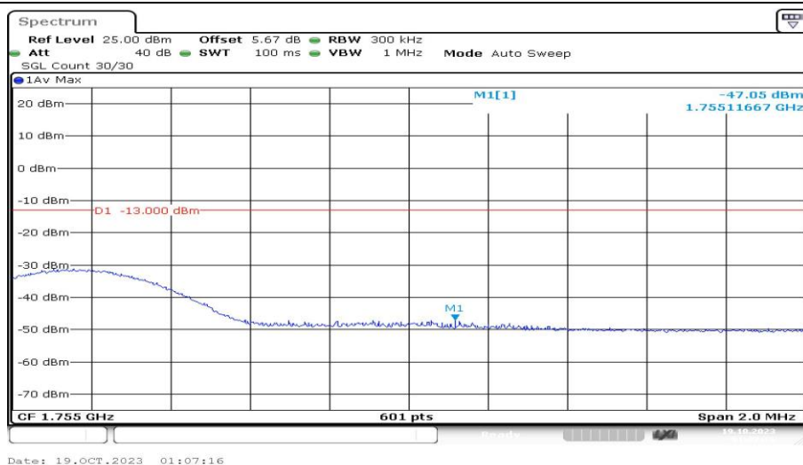
Band4-15MHz-16QAM-20325-1RB#0-PASS
