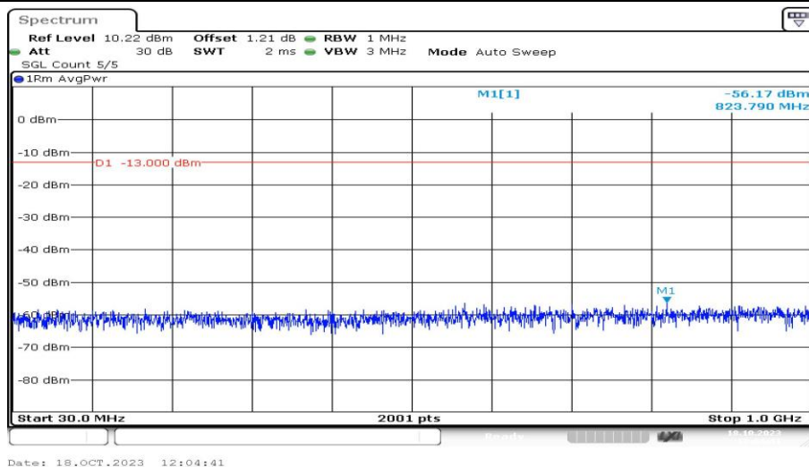
Band4-1.4MHz-QPSK-20393-1RB#0-Range3:30~1000MHz-PASS
