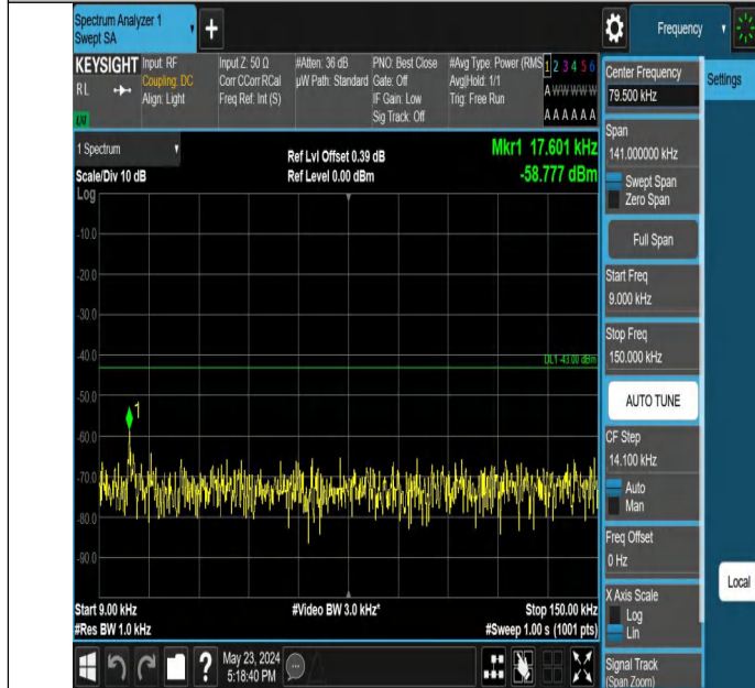
Band2_5MHz_QPSK_18900_1RB#0_0.009~0.15_0.009~0.15
