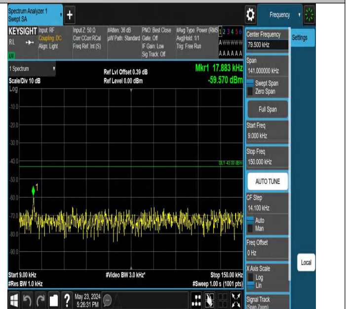
Band2_10MHz_QPSK_19150_1RB#49_0.009~0.15_0.009~0.15
