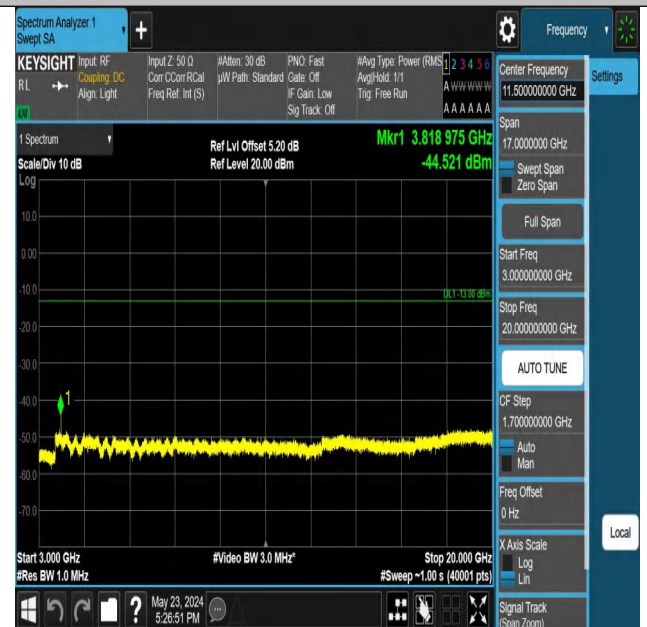
Band2_10MHz_QPSK_19150_1RB#49_3000~20000_3000~20000
