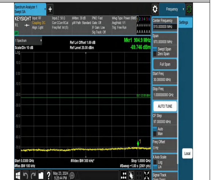
Band2 10MHz QPSK 18900 1RB#49 30~1000 30~1000
