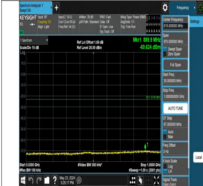
Band2_10MHz_QPSK_18900_1RB#0_30~1000_30~1000
