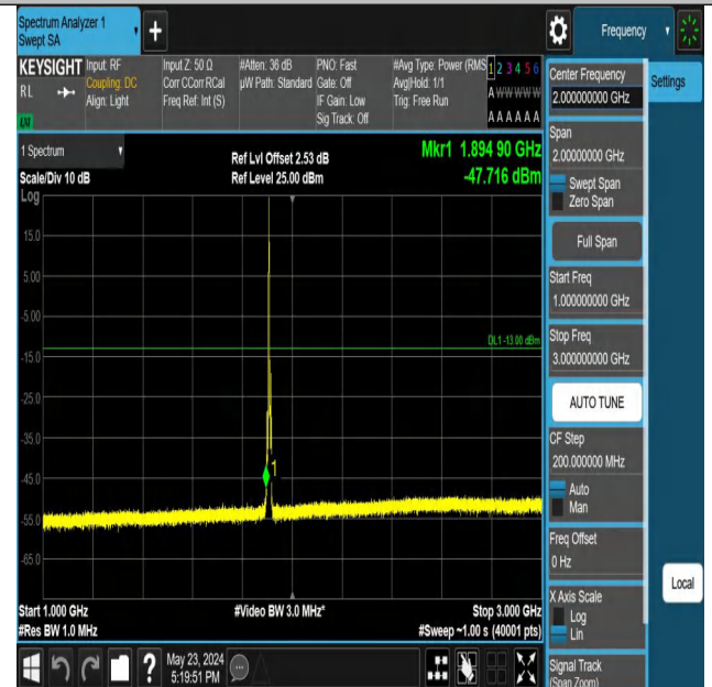
Band2_5MHz_QPSK_19175_1RB#0_1000~3000_1000~3000
