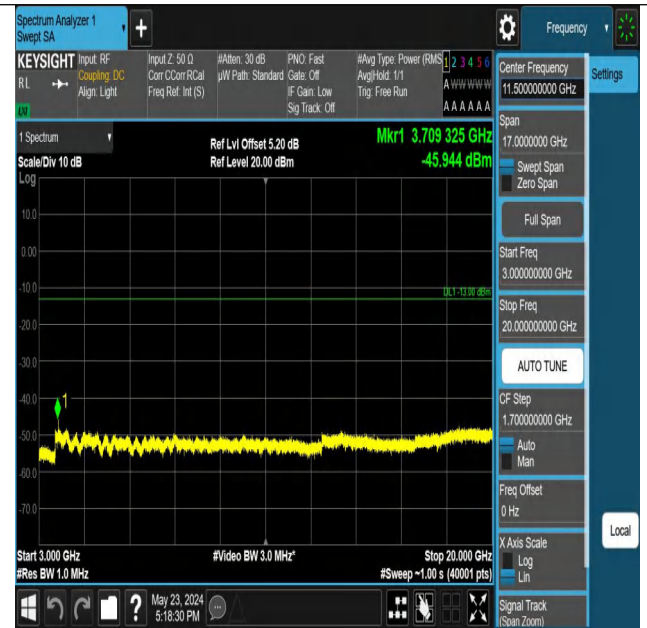
Band2_5MHz_QPSK_18625_1RB#24_3000~20000_3000~20000
