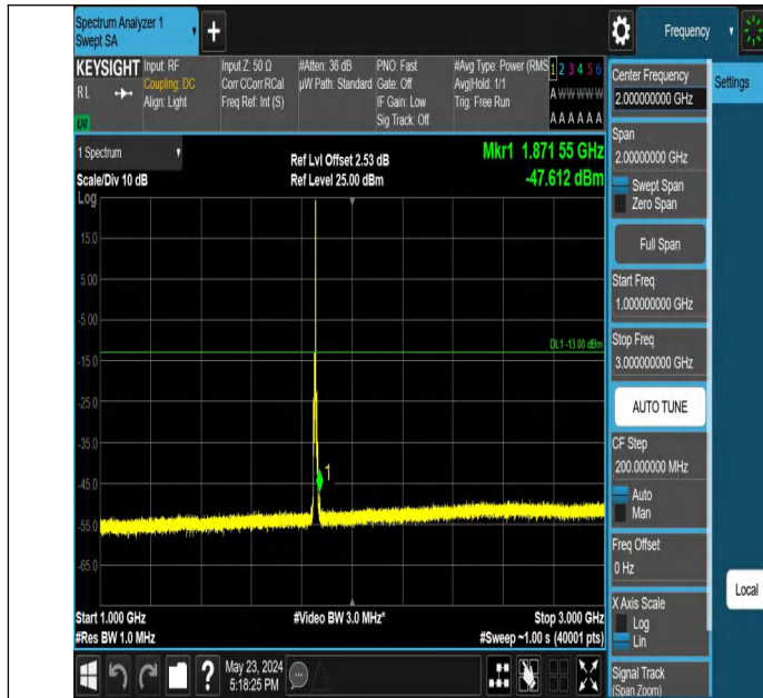
Band2_5MHz_QPSK_18625_1RB#24_1000~3000_1000~3000
