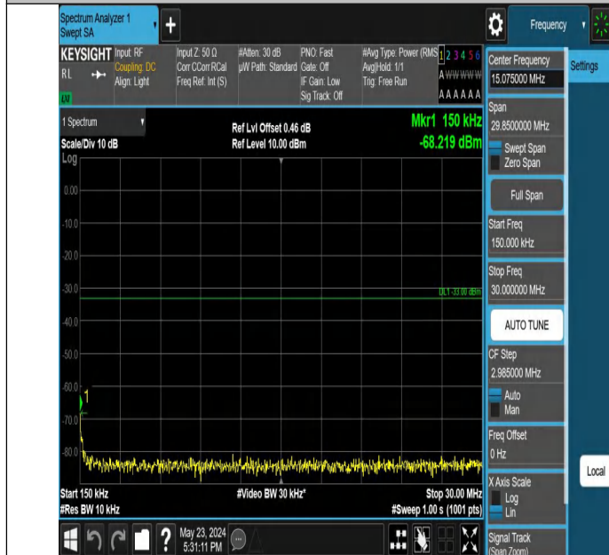
Band2_15MHz_QPSK_18675_1RB#74_0.15~30_0.15~30
