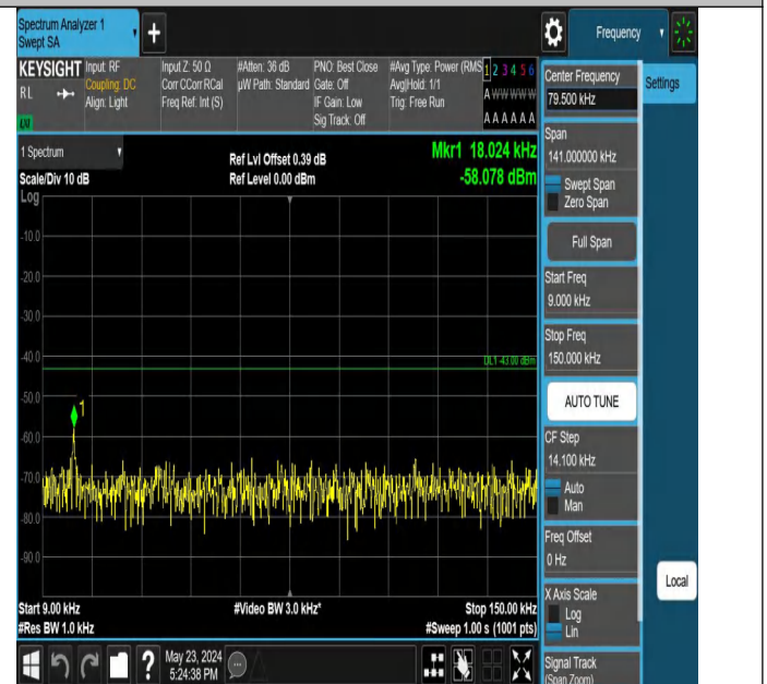
Band2_10MHz_QPSK_18650_1RB#49_0.009~0.15_0.009~0.15
