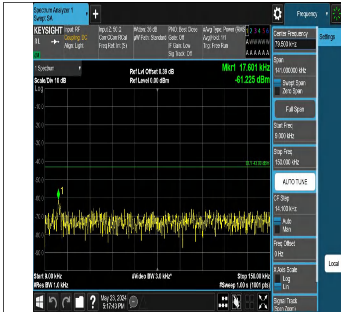
Band2_5MHz_QPSK_18625_1RB#0_0.009~0.15_0.009~0.15
