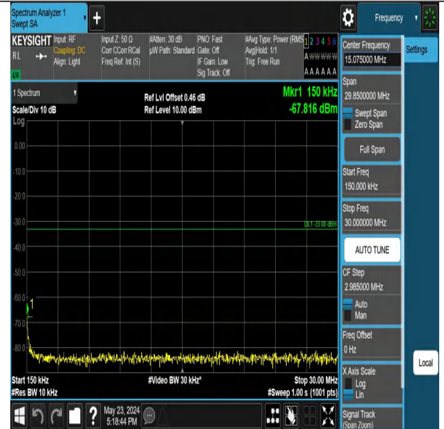
Band2_5MHz_QPSK_18900_1RB#0_0.15~30_0.15~30
