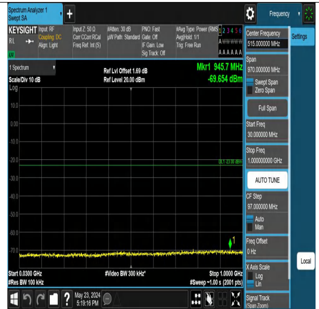
Band2_5MHz_QPSK_18900_1RB#24_30~1000_30~1000
