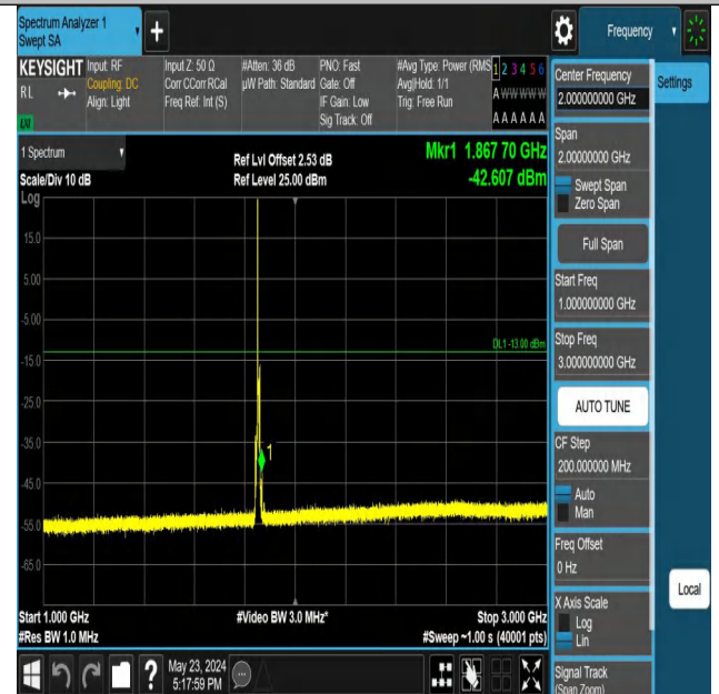
Band2_5MHz_QPSK_18625_1RB#0_1000~3000_1000~3000
