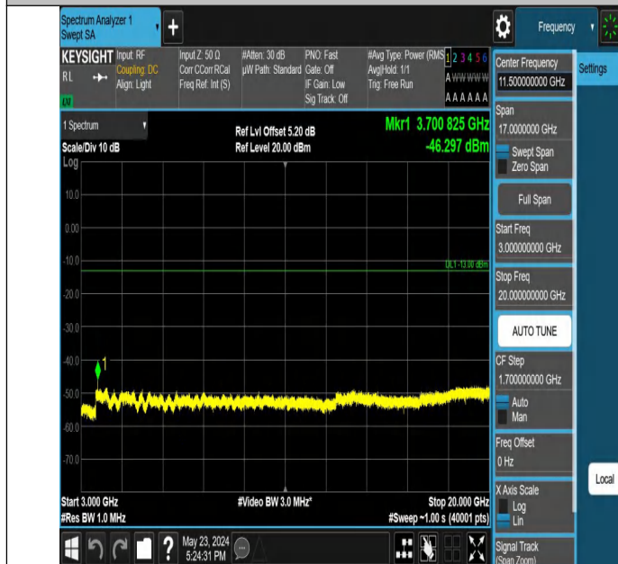
Band2_10MHz_QPSK_18650_1RB#0_3000~20000_3000~20000
