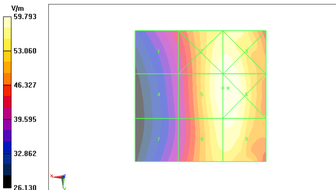
Fig B.9 HAC RF E-Field WCDMA 850 Low
