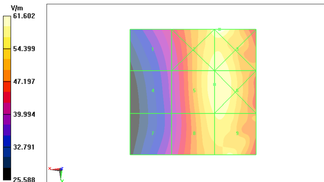
Fig B.8 HAC RF E-Field WCDMA 850 Middle
