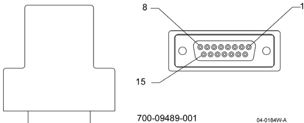
700-09489-xxx SIM Rectifier Alarm Mask Connector
