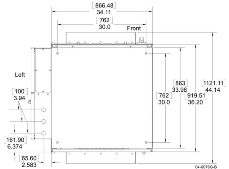
Cabinet Bottom
