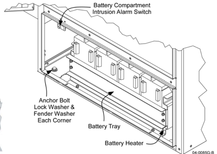
Frame Mounting
