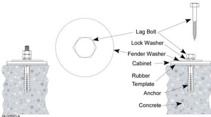
Frame Mounting
