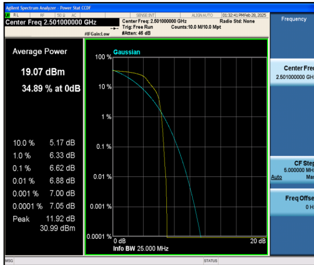
Band41-10MHz-QPSK-39700-1RB#0-PASS
