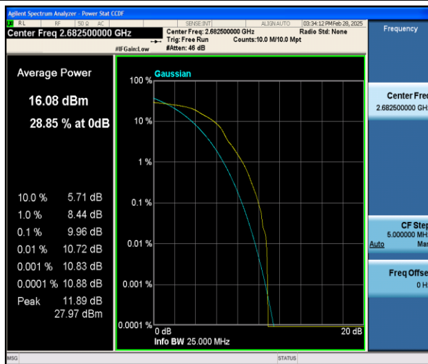
Band41-15MHz-16QAM-41515-1RB#0-PASS
