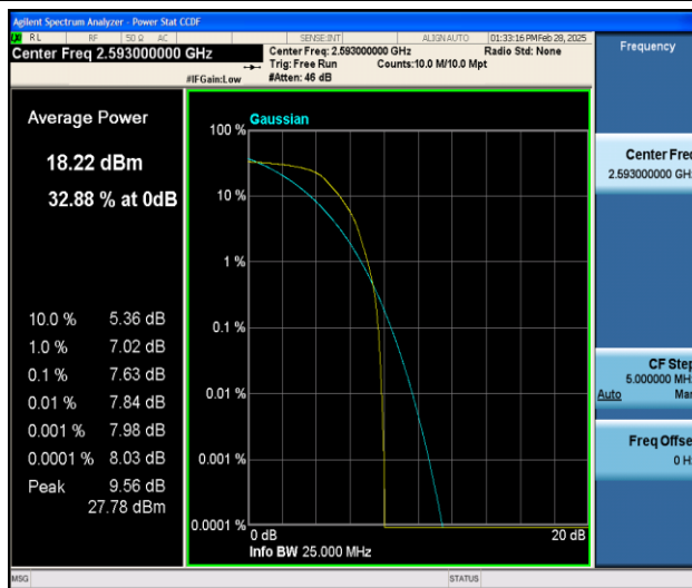
Band41-10MHz-QPSK-40620-1RB#0-PASS
