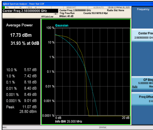
Band41-20MHz-16QAM-40620-1RB#0-PASS
