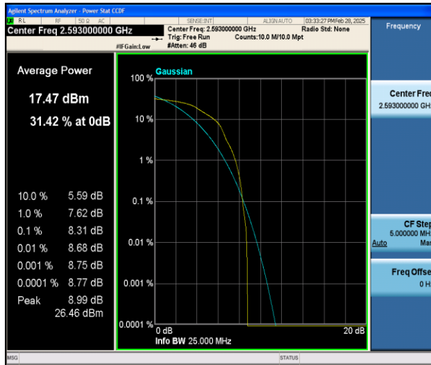
Band41-15MHz-16QAM-40620-1RB#0-PASS
