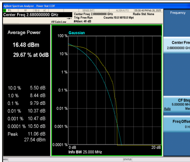
Band41-20MHz-16QAM-41490-1RB#0-PASS
