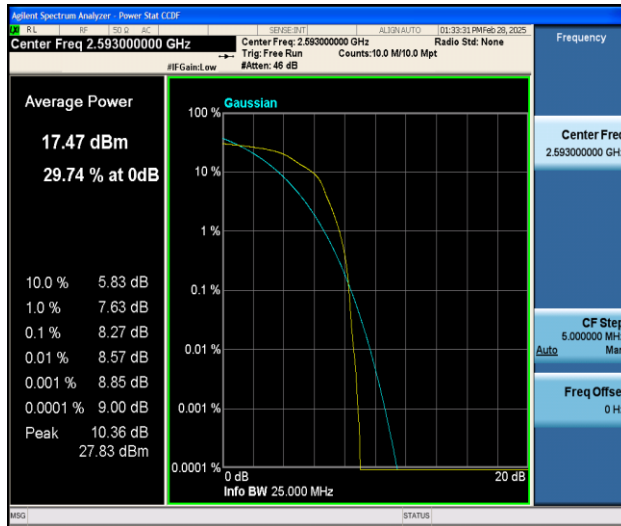
Band41-10MHz-16QAM-40620-1RB#0-PASS
