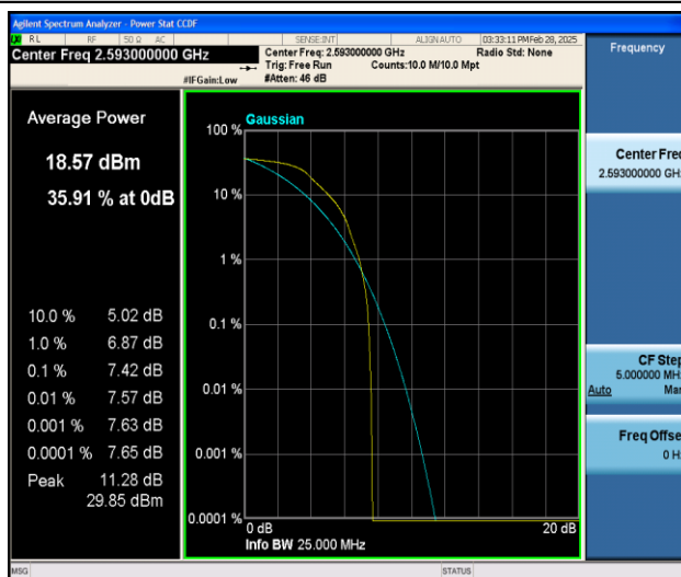
Band41-15MHz-QPSK-40620-1RB#0-PASS
