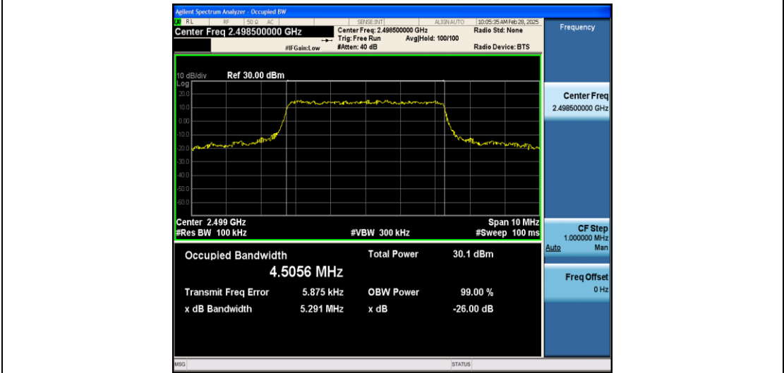
Band41-5MHz-16QAM-39675-25RB#0-PASS
