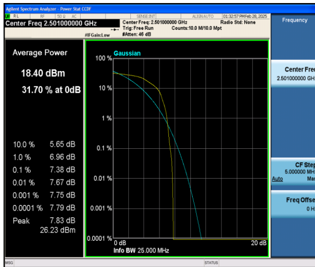
Band41-10MHz-16QAM-39700-1RB#0-PASS
