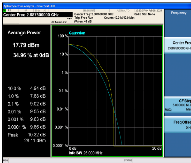
Band41-5MHz-QPSK-41565-1RB#0-PASS
