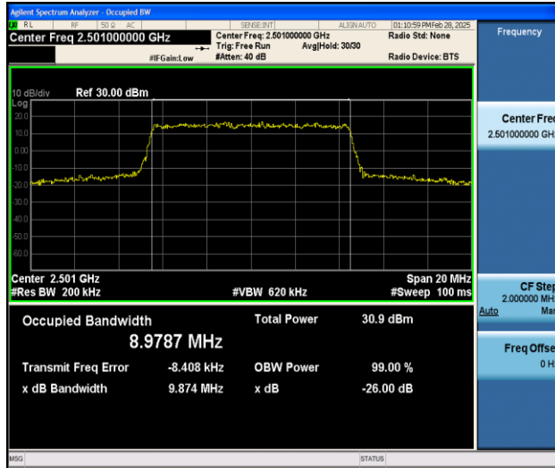
Band41-10MHz-QPSK-39700-50RB#0-PASS
