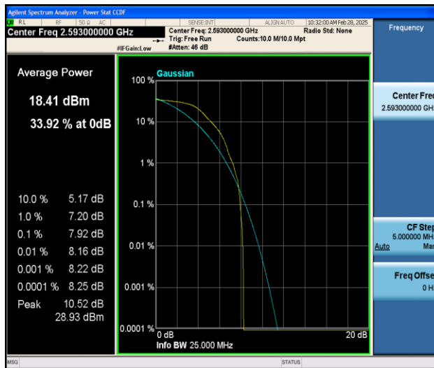
Band41-5MHz-QPSK-40620-1RB#0-PASS
