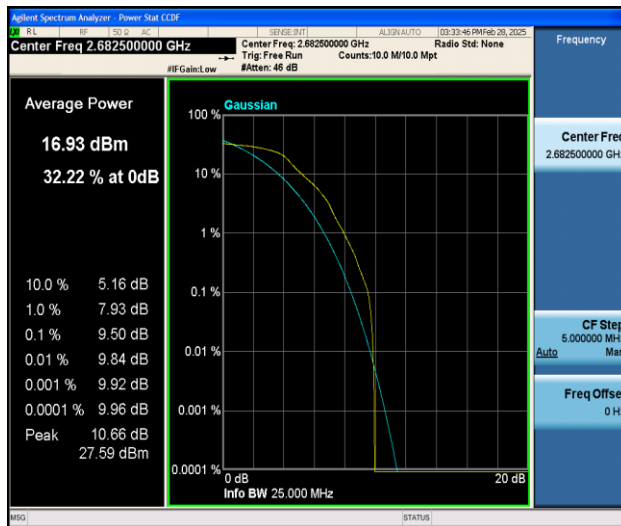
Band41-15MHz-QPSK-41515-1RB#0-PASS
