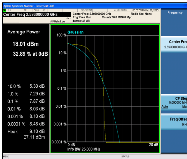
Band41-20MHz-QPSK-40620-1RB#0-PASS
