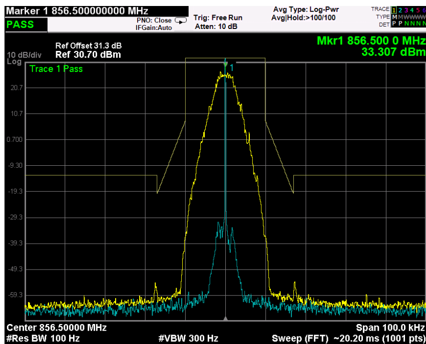
Mask G
