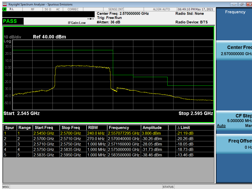
Plot 7-21. Upper ACP Plot (LTE Band 7 - 15MHz QPSK – Full RB)
