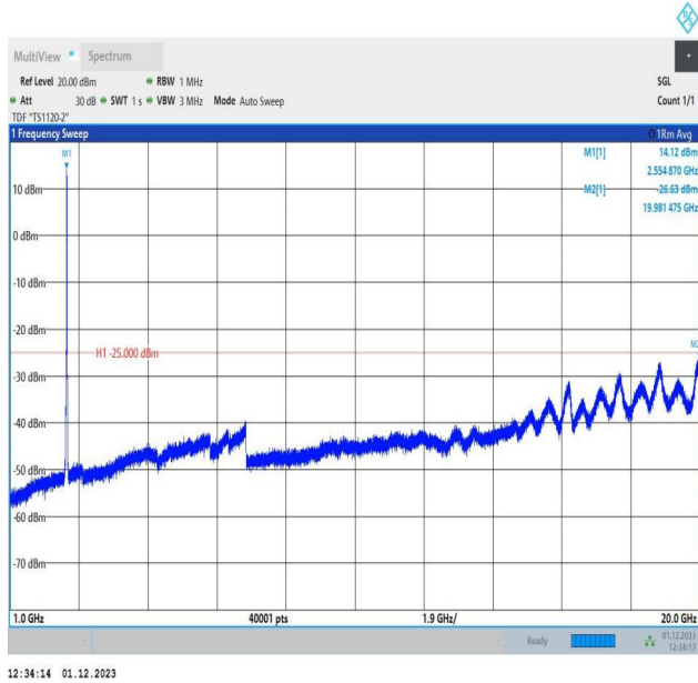
7-7-15MHz-5MHz-64QAM-64QAM-21327-21420-75RB#0-25R B#0-1000~20000MHz-PASS
