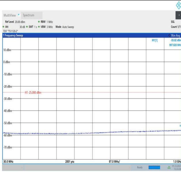
7-7-15MHz-5MHz-16QAM-16QAM-21327-21420-75RB#0-25R B#0-30~1000MHz-PASS
