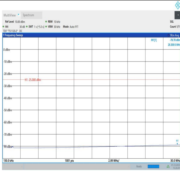
7-7-10MHz-20MHz-64QAM-64QAM-20805-20949-50RB#0-10 ORB#0-0.15~30MHz-PASS
