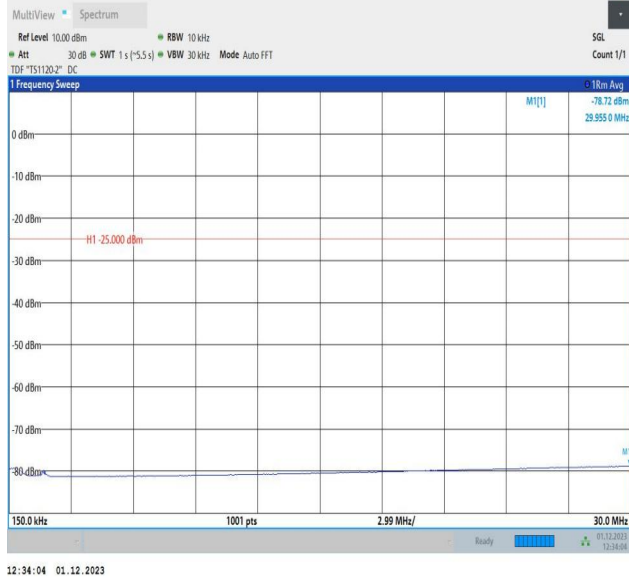
7-7-15MHz-5MHz-64QAM-64QAM-21327-21420-75RB#0-25R B#0-0.15~30MHz-PASS
