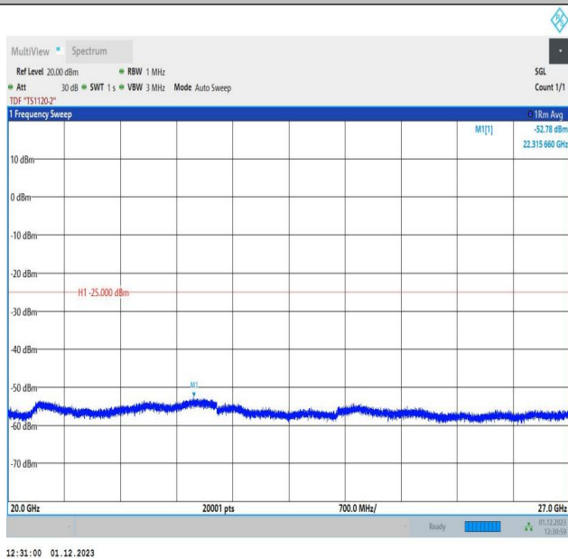
7-7-15MHz-5MHz-QPSK-QPSK-21327-21420-1RB#0-1RB#24 -20000~27000MHz-PASS
