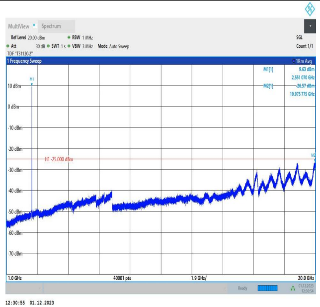
7-7-15MHz-5MHz-QPSK-QPSK-21327-21420-1RB#0-1RB#24 -1000~20000MHz-PASS
