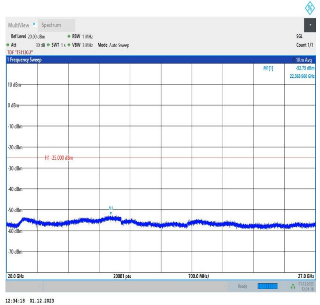
7-7-15MHz-5MHz-64QAM-64QAM-21327-21420-75RB#0-25R B#0-20000~27000MHz-PASS
