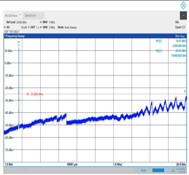
7-7-15MHz-5MHz-16QAM-16QAM-21327-21420-75RB#0-25R B#0-1000~20000MHz-PASS
