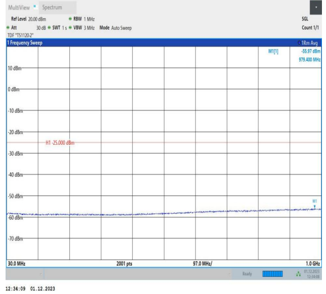
7-7-15MHz-5MHz-64QAM-64QAM-21327-21420-75RB#0-25R B#0-30~1000MHz-PASS
