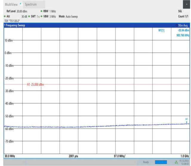
7-7-15MHz-5MHz-QPSK-QPSK-21327-21420-1RB#74-0RB#0 -30~1000MHz-PASS
