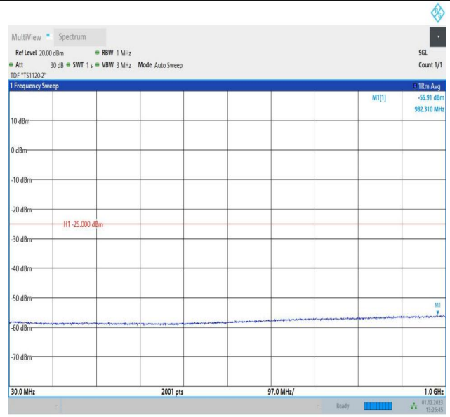
7-7-10MHz-20MHz-64QAM-64QAM-20805-20949-50RB#0-10 ORB#0-30~1000MHz-PASS
