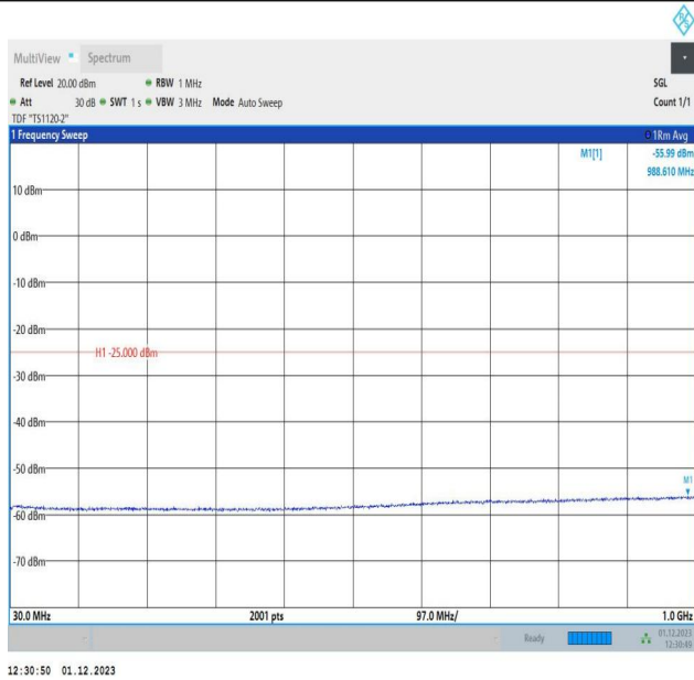
7-7-15MHz-5MHz-QPSK-QPSK-21327-21420-1RB#0-1RB#24 -30~1000MHz-PASS
