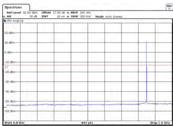
LTE Band 5 1.4MHz CH-High 9kHz~1GHz
