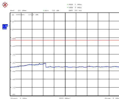
LTE Band 5 1.4MHz CH-High 1GHz~9GHz
