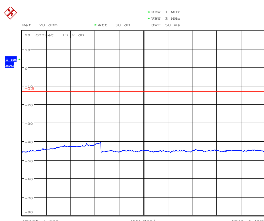
LTE Band 5 1.4MHz CH-Middle 1GHz~9GHz
