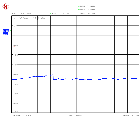
LTE Band 5 1.4MHz CH-Low 1GHz~9GHz
