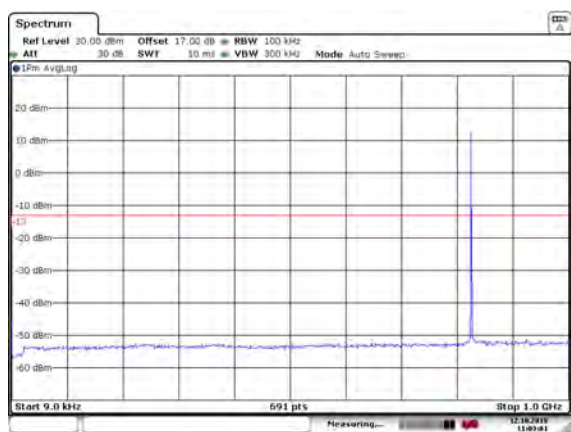
LTE Band 5 1.4MHz CH-Low 9kHz~1GHz
