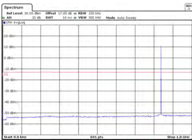
LTE Band 5 1.4MHz CH-Middle 9kHz~1GHz
