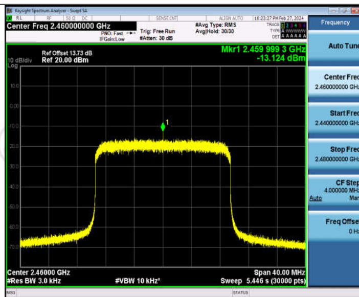
2.4G Slot 20MHz Ant2 2460
