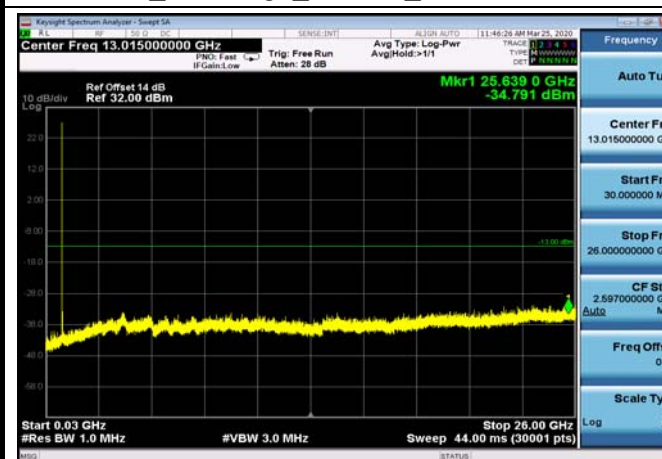
FDD26_MidRange_15MHz_30MHz~26GHz
