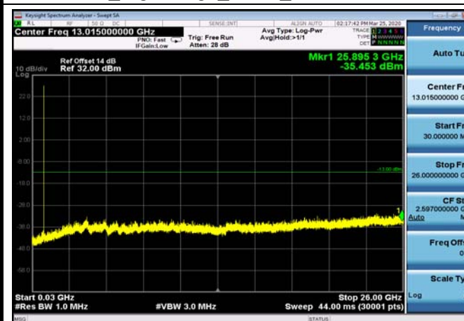
FDD26_HighRange_5MHz_30MHz~26GHz
