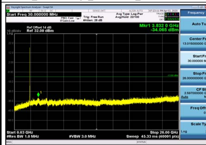
FDD7_LowRange_15+15MHz_30MHz~26GHz
