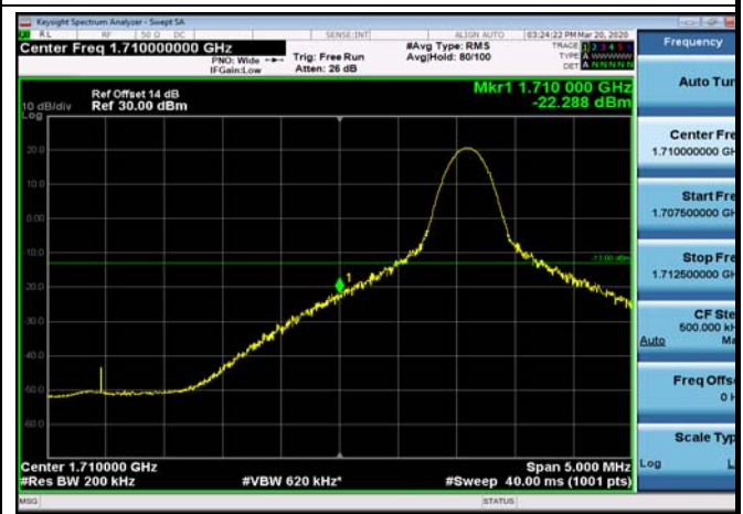
LowRange_FDD04_20MHz_1720_OneRB _low_Q16
