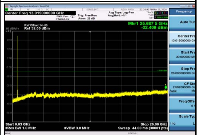
FDD26_MidRange_3MHz_30MHz~26GHz
