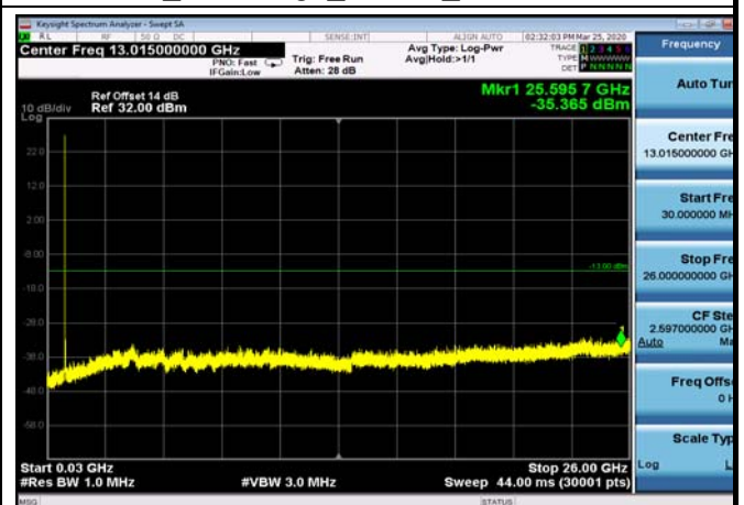
FDD26_LowRange_15MHz_30MHz~26GHz
