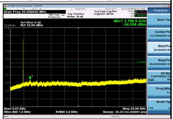
FDD7_MiddleRange_15+15MHz_30MHz~26GHz
