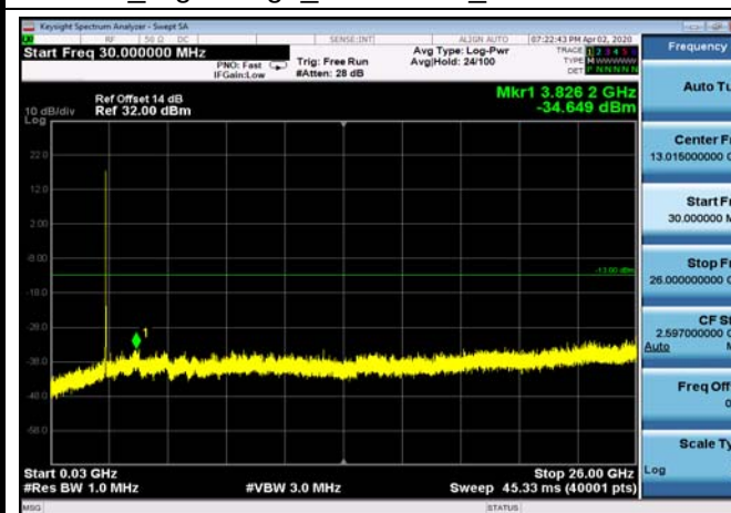
FDD7_HighRange_20+20MHz_30MHz~26GHz
