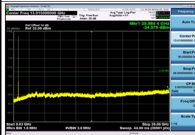
FDD26_HighRange_15MHz_30MHz~26GHz
