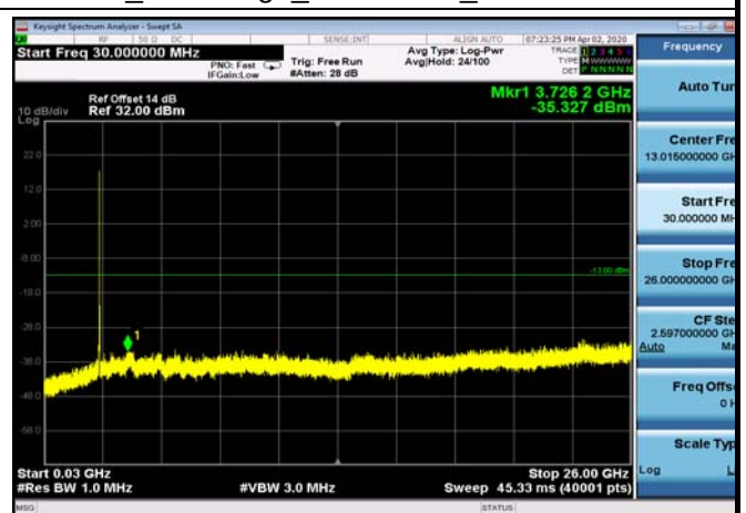
FDD7_LowRange_20+15MHz_30MHz~26GHz
