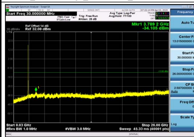
FDD7_LowRange_20+20MHz_30MHz~26GHz
