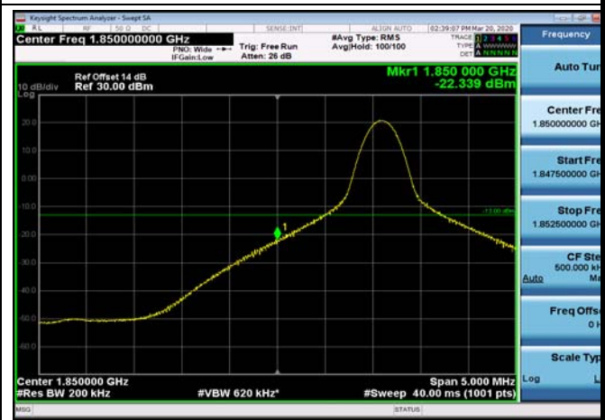
LowRange_FDD02_20MHz_1860_OneRB _low_Q16
