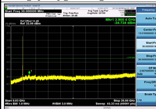
FDD7_HighRange_15+15MHz_30MHz~26GHz
