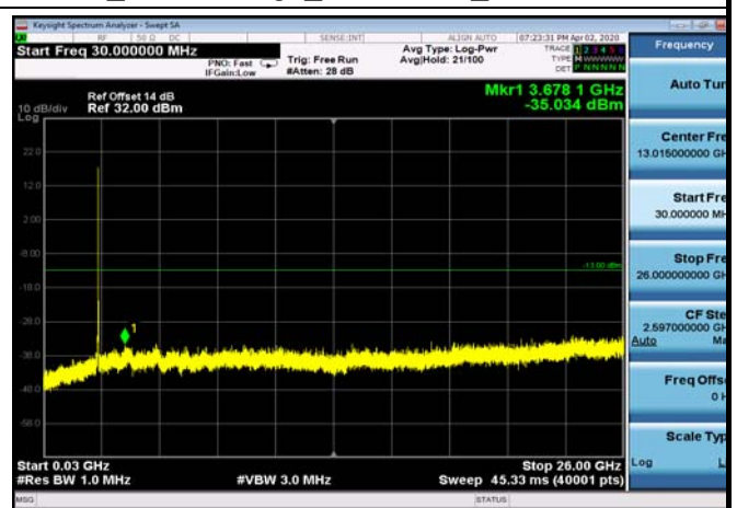
FDD7_LowRange_15+10MHz_30MHz~26GHz
