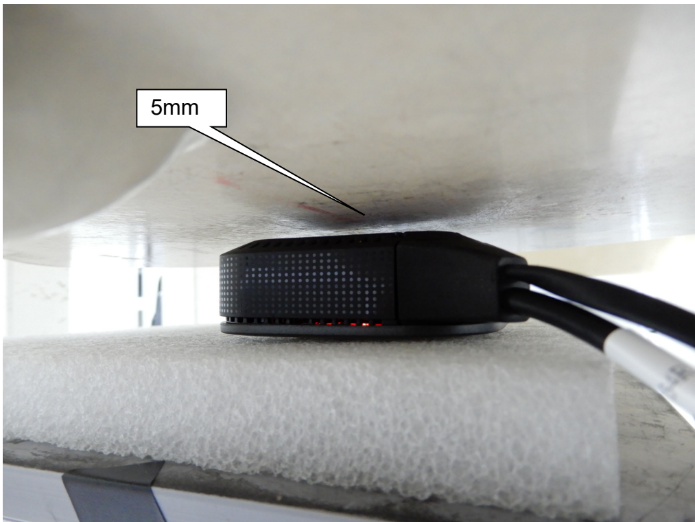
EUT Back_5mm
