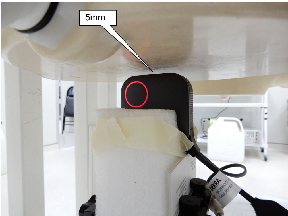
EUT Right-side_5mm
