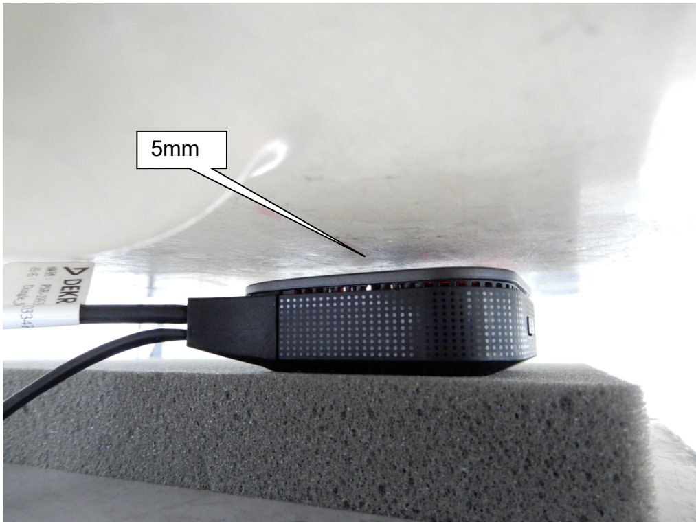
EUT Front_5mm
