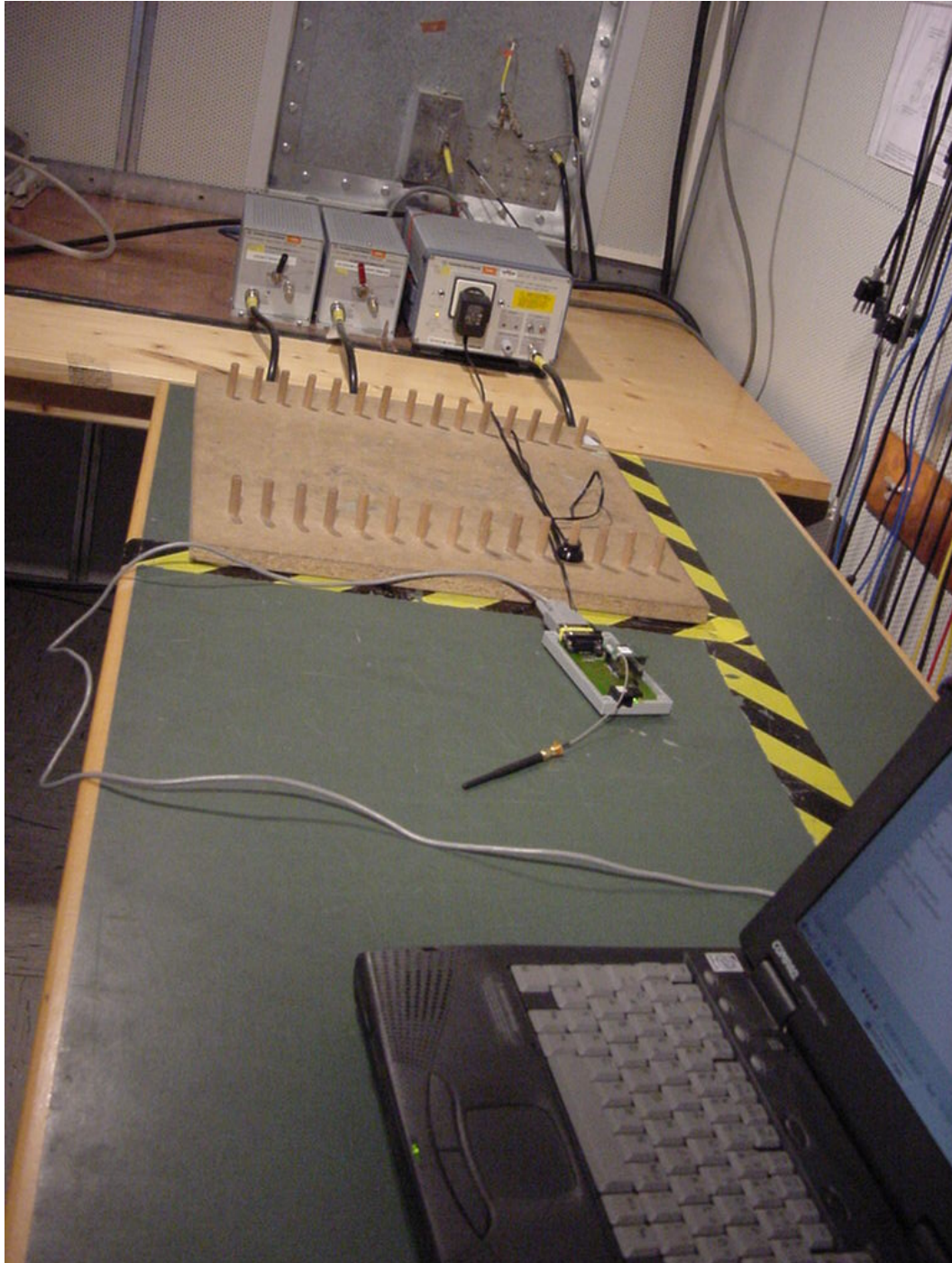
Photo 3: Conducted Emissions
