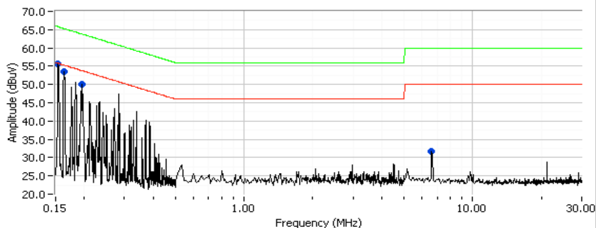
DC Power Port Conducted Emissions, 0.15 - 30MHz (Line)
