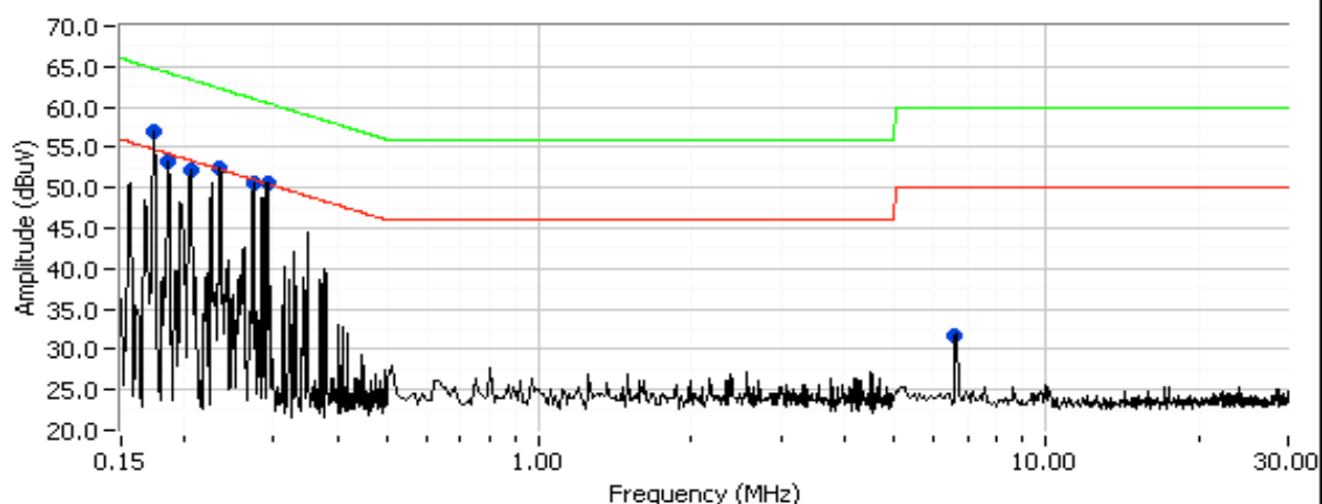
DC Power Port Conducted Emissions, 0.15 - 30MHz (Return)
