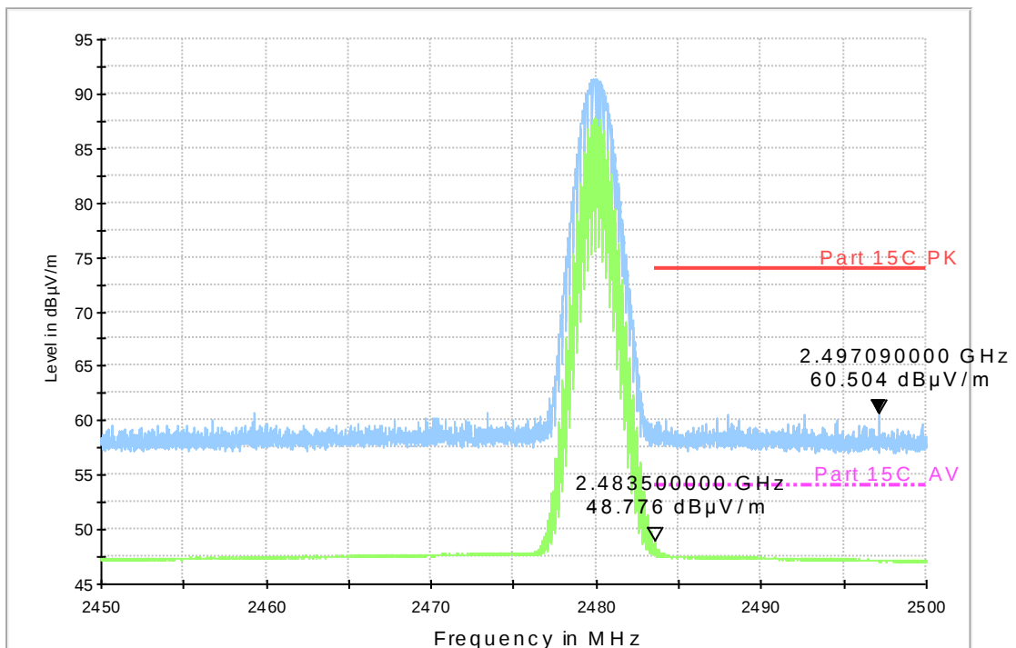
Radiated emission (Power): 8DPSK, high channel
