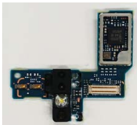
Internal Sub-PWB without Shield cases (Front-side)
