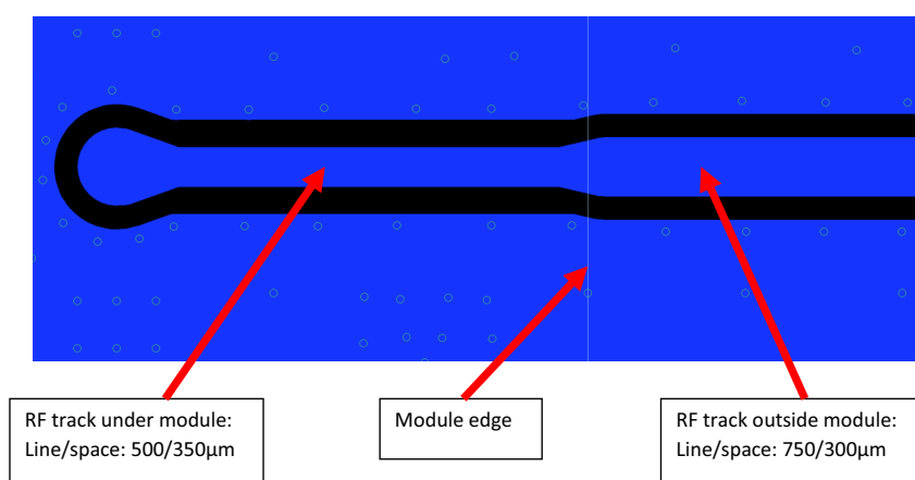
Figure 10: Routing detail
