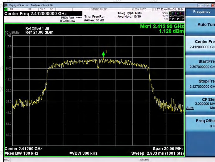
11N20SISO-Ant1-2412-0~Reference-PASS
