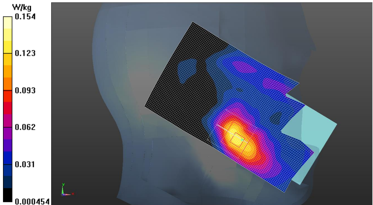
Fig.29 LTE Band 25
