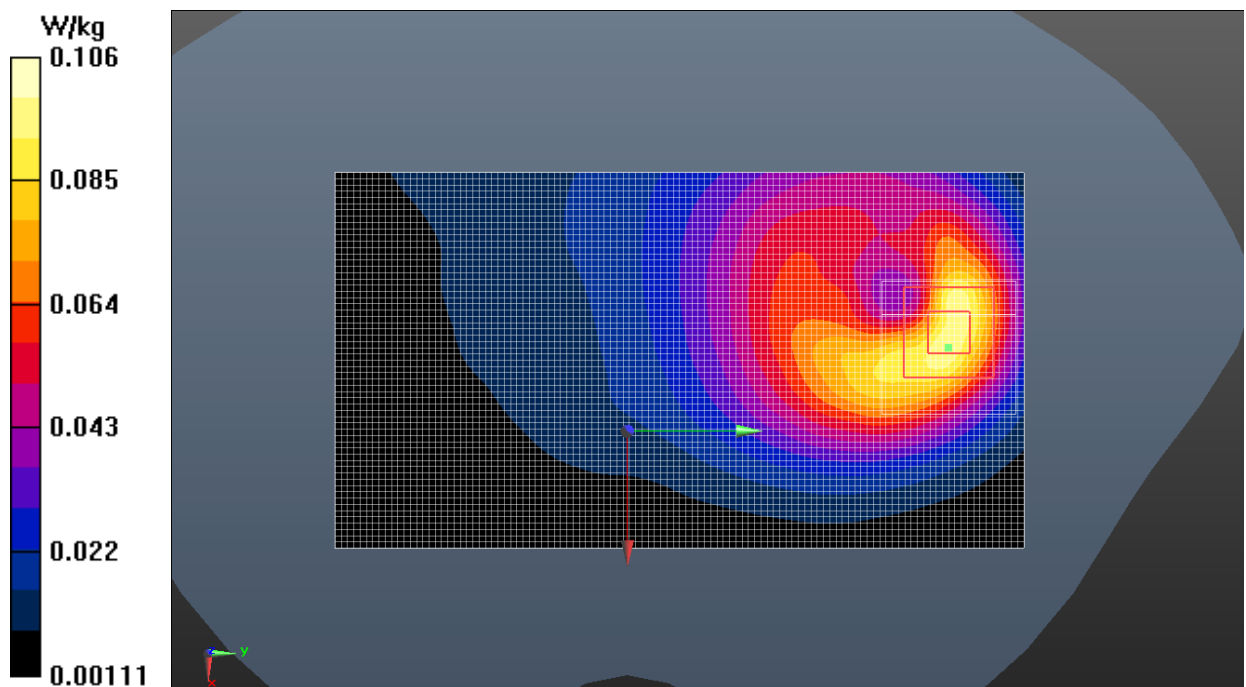
Fig.38 LTE Band 71
