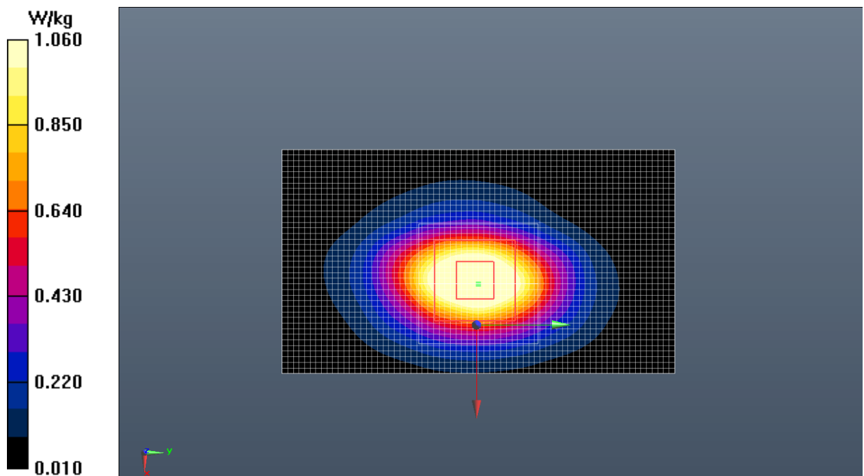
Fig.30 LTE Band 25
