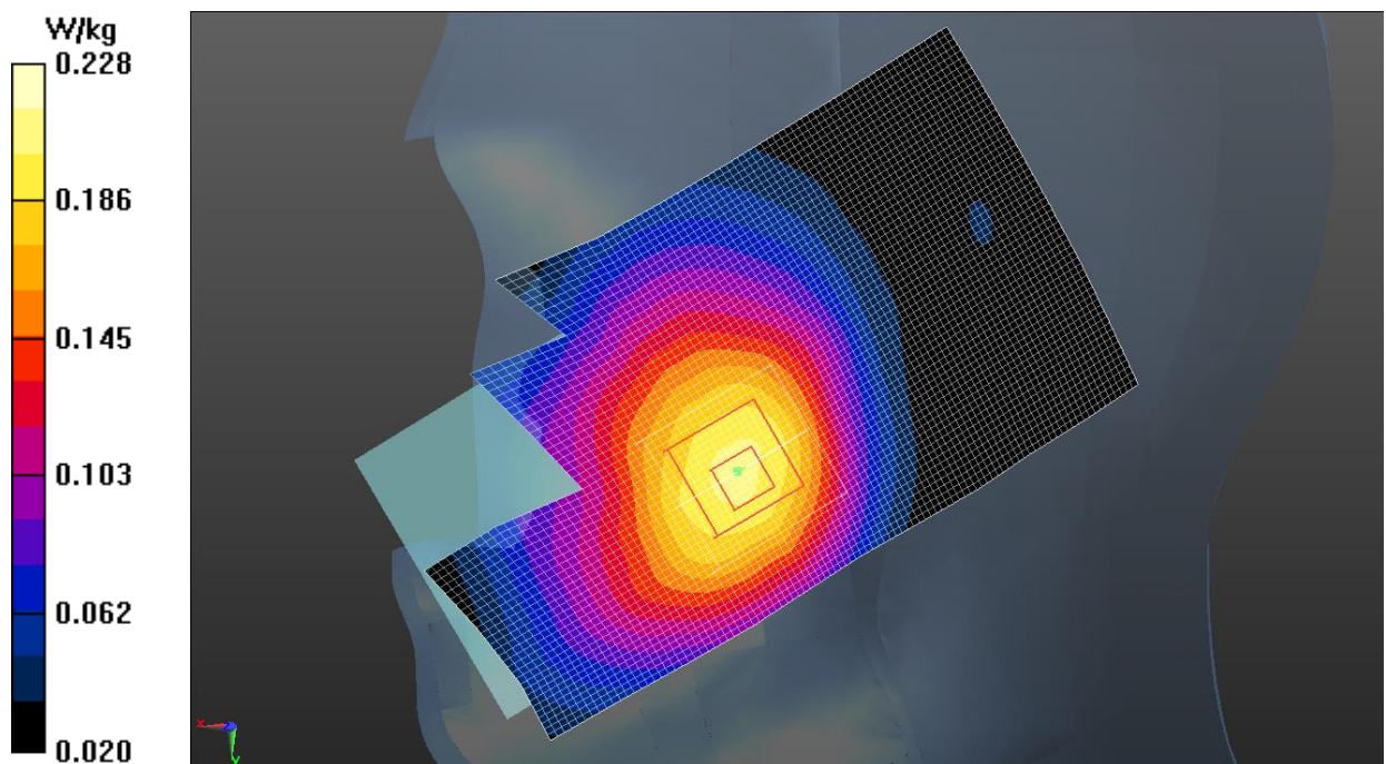
Fig.31 LTE Band 26
