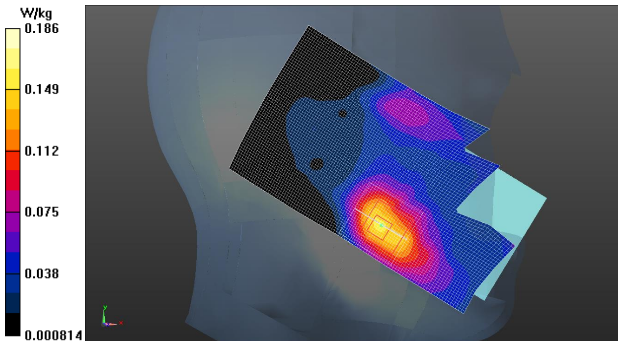
Fig.35 LTE Band 66
