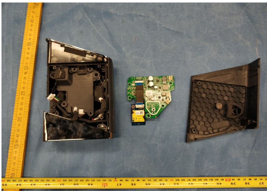
Internal View of EUT-18 surround (left)
