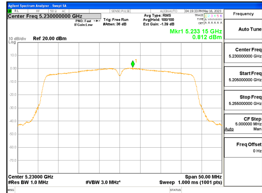
ANT L_802.11ac_VHT40_UNII 1
