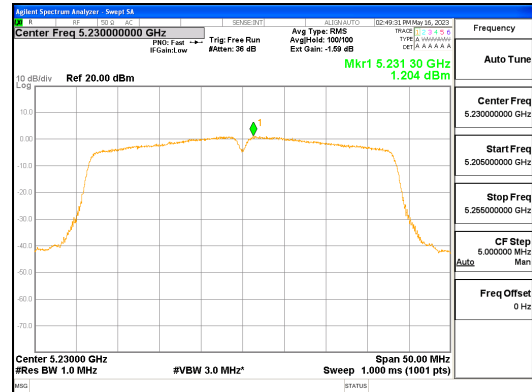
ANT R_802.11n_HT40_UNII 1
