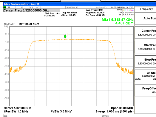
ANT L_802.11ax_HE20_242T_UNII 2A
