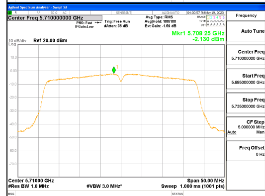
ANT R_802.11ac_VHT40_UNII 2C
