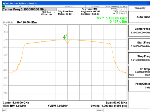
ANT R_802.11n_HT40_UNII 1
