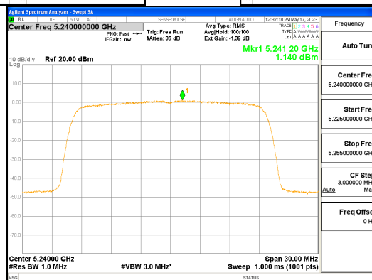
ANT L_802.11ax_HE20_242T_UNII 1
